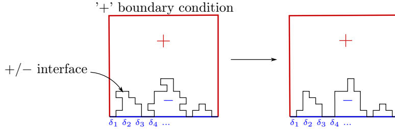
Figure 2.3 – Schematic view of the +/- interface in the Ising model with '+ boundary condition on three sides and '- on the last side of the square. On the right is the effective interface, which is modeled by a random walk conditioned to stay non-negative and to return to 0.
