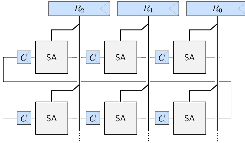
Figure 4.7: Kulisch-3 accumulator, here for S = 3 .
