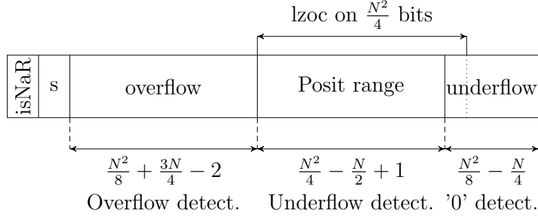
Figure 5.7: Quire conversion to posit intermediate format .
