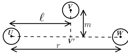
Figure 4.1: Three disks with centers \mathbf{U} , \mathbf{V} and \mathbf{W} .
