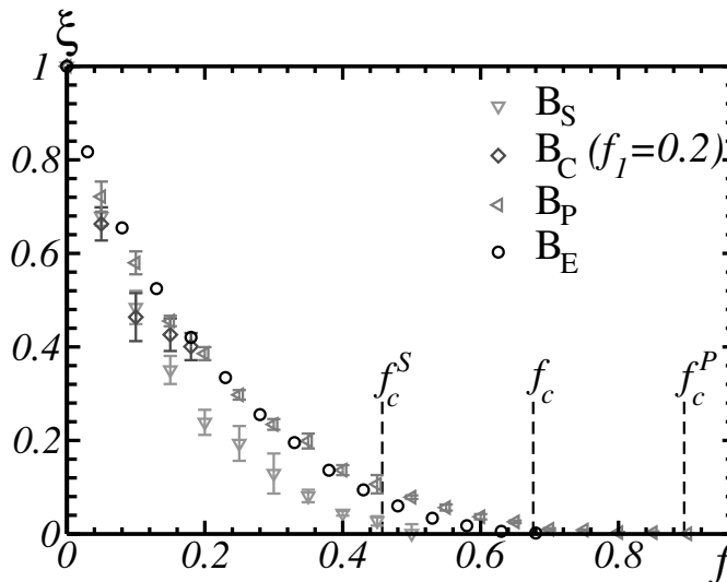
Figure 6.2: Length of minimal paths in the Boolean model \mathcal{B}_E (black circles) and in various two-scale Boolean models: \mathcal{B}_P (left triangles), \mathcal{B}_C (diamonds) and \mathcal{B}_S (bottom triangles).
