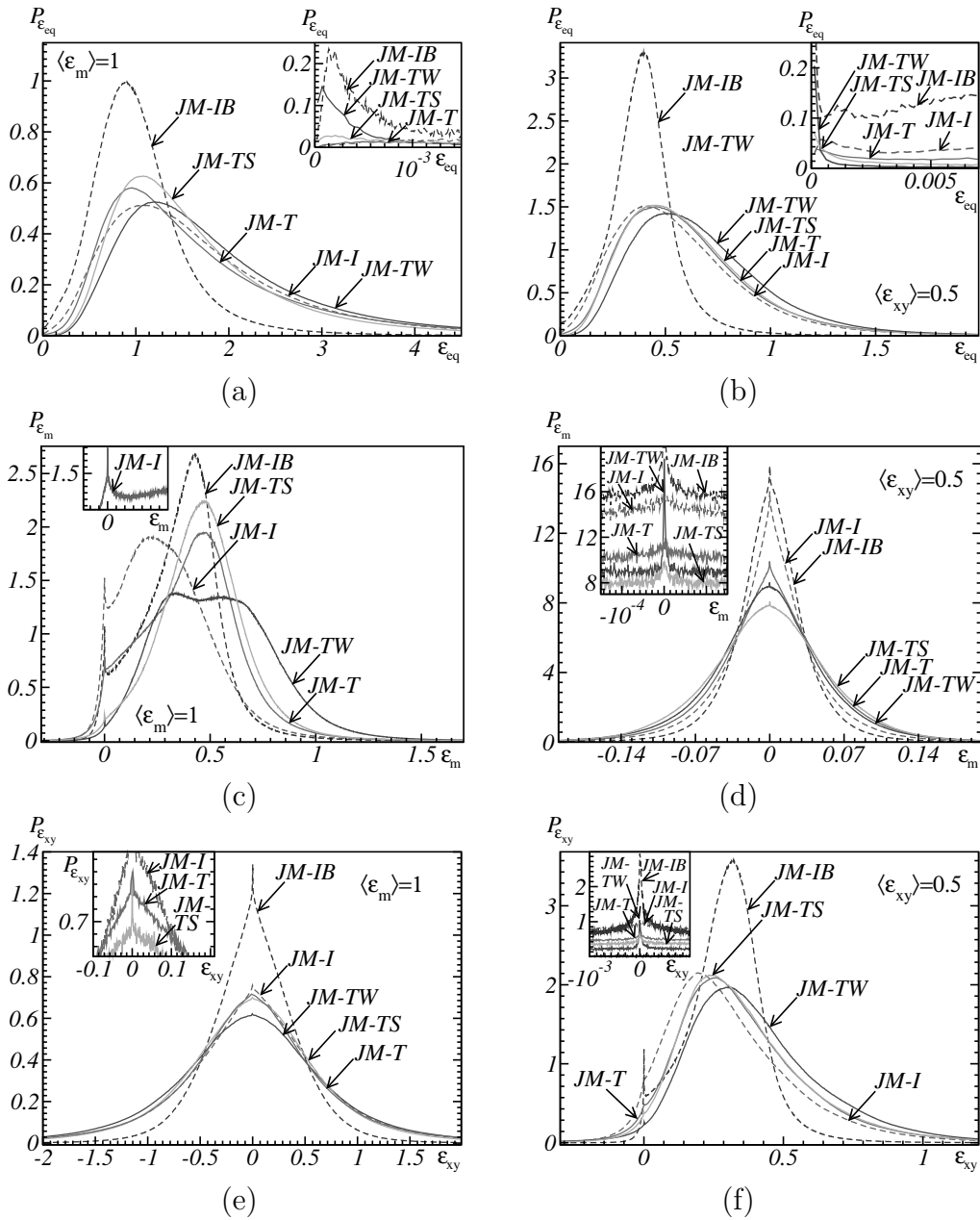
Figure 3.11: Histograms of the strain field components \epsilon_{eq} (a,b), \epsilon_m (c,d), \epsilon_{xy} (e,f) in various cracked media, subjected to hydrostatic strain loading (a,c,e) or shear (b,d,f). JM-I: polycrystal with intergranular cracks. JM-T: transgranular cracks. JM-TW: “weak-plane” transgranular cracks. JM-TS: “stiff-plane” transgranular cracks. JM-IB: homogeneous cracked body. Embedded graphs: strain distribution in the region \epsilon \approx 0 .
