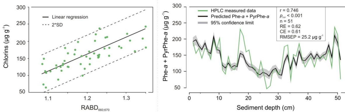
Fig. 3. Proxy-proxy calibration models with associated scatterplots and downcore comparison: a between compound-specific HPLC pigments and UV-VIS measurements; b between HPLC sedimentary pigments and VIS-RS logging
