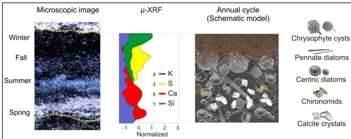
Fig. 5.7 Microscopic image of a thin section, \mu -XRF data, and a schematic model of an annual sediment deposition in Lake Żabińskie
