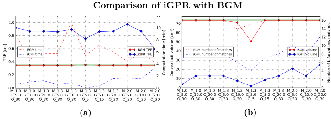
Figure V.1: Accuracy and search space using different Mahalanobis (M), Geodesic (G) and Outliers (O) thresholds. In a) The TRE is plotted in solid lines. The iGPR (in blue) although is fast it is far from the ground truth (green thick horizontal line) and has high variability on the parameters used. The BGM TRE (in red) converges to the coarse TRE ground truth. In b) Similarly, the BGM convex hull volume and its number of bifurcations mostly converge to the ground truth values.
