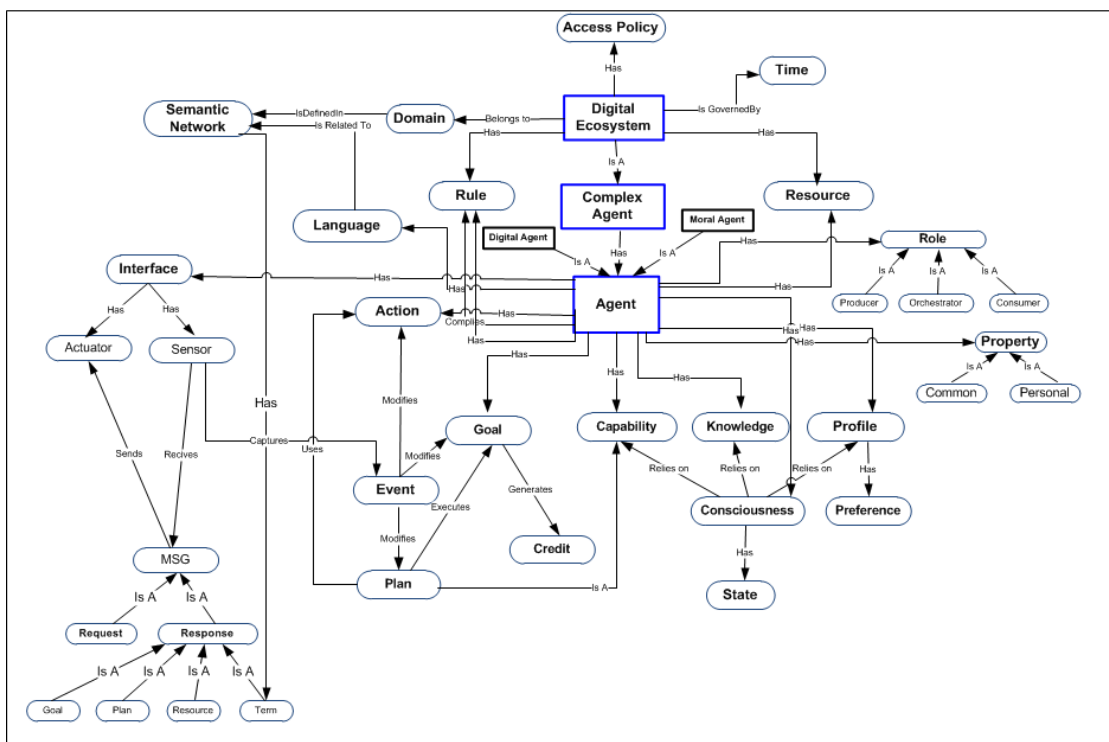
FIGURE 3.7: Detailed Conceptual Model for MAS-based Digital Ecosystem
