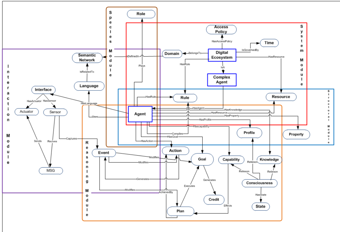
FIGURE 3.1: Conceptual Model for MAS-based Digital Ecosystem
