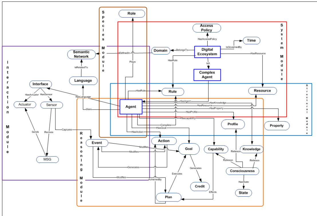
FIGURE 4.2: MAS2DES-Onto Conceptual Model
