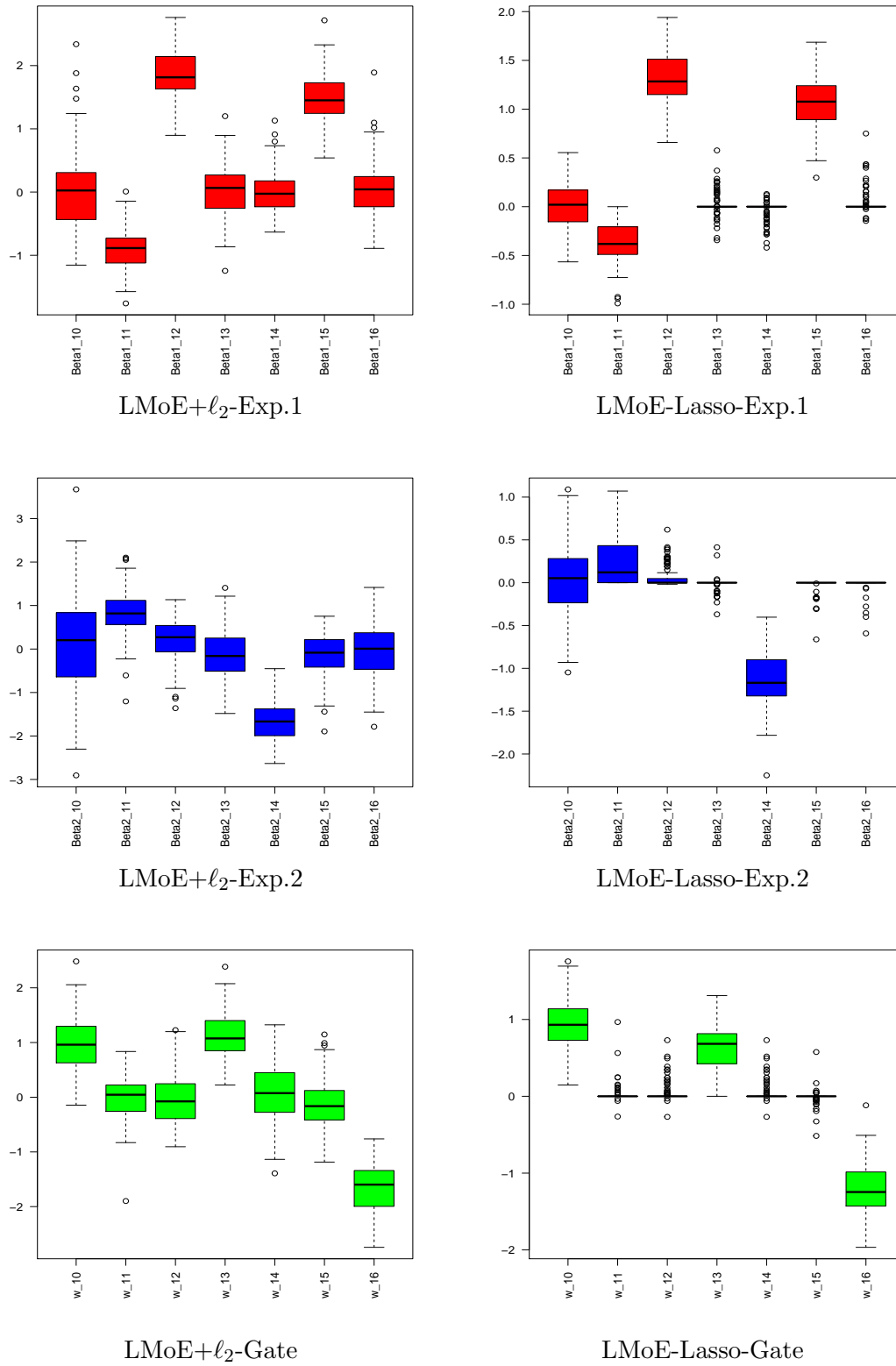
Figure 4.3: Boxplots of l_2 regularized MoE model (LMoE+ l_2 ) and the proposed Lasso penalized MoE model (LMoE-Lasso) for logistic case.
