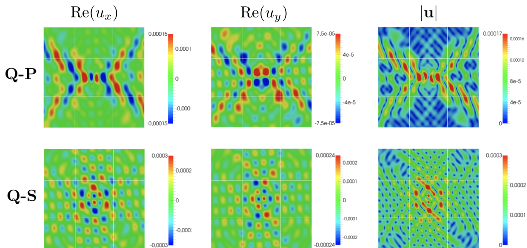
Figure 2.8: Anisotropic case : we represent \text{Re}u_x (left), \text{Re}u_y (center) and |\mathbf{u}| (right) for a source term with a null rotational (first line, Quasi-P wave) and with a null divergence (second line, Quasi-S wave).
