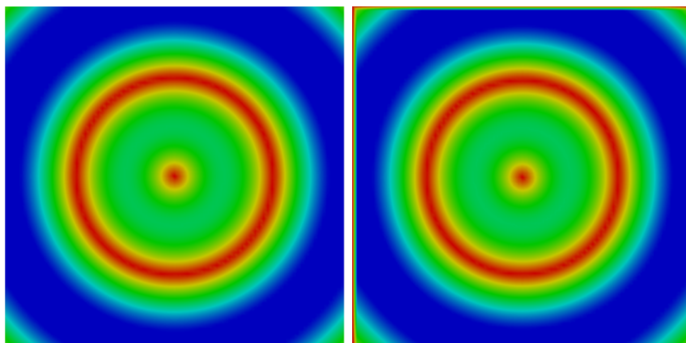
Figure 2.9: Isotropic case : we represent |\mathbf{u}| computed with the HsMM (left) and the PML (right).
