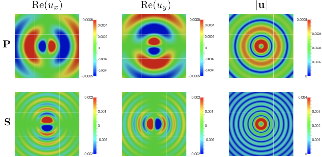
Figure 2.7: Isotropic case : we represent \operatorname{Re}u_x (left), \operatorname{Re}u_y (center) and |u| (right) for a source term with a null rotational (first line, P wave) and with a null divergence (second line, S wave).
