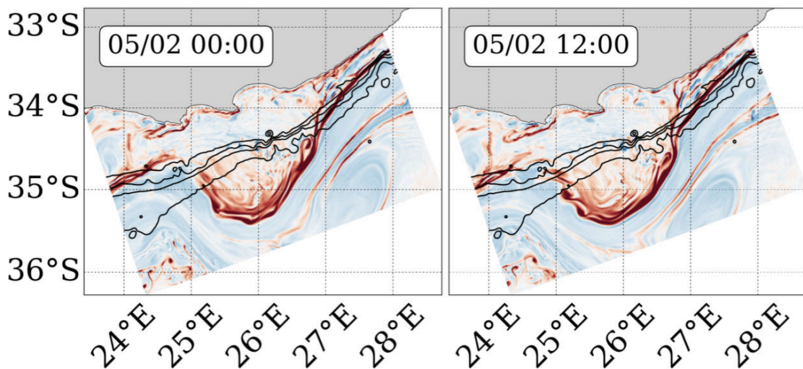
Figure 2.66 – Maps of surface normalized vertical relative vorticity (values between \pm 2f ) at snapshots during a Natal Pulse event when submesoscale eddies were seen to develop. Black lines represent the 200, 500, 1000 and 2000 m isobaths. Figure from P. Tedesco.
