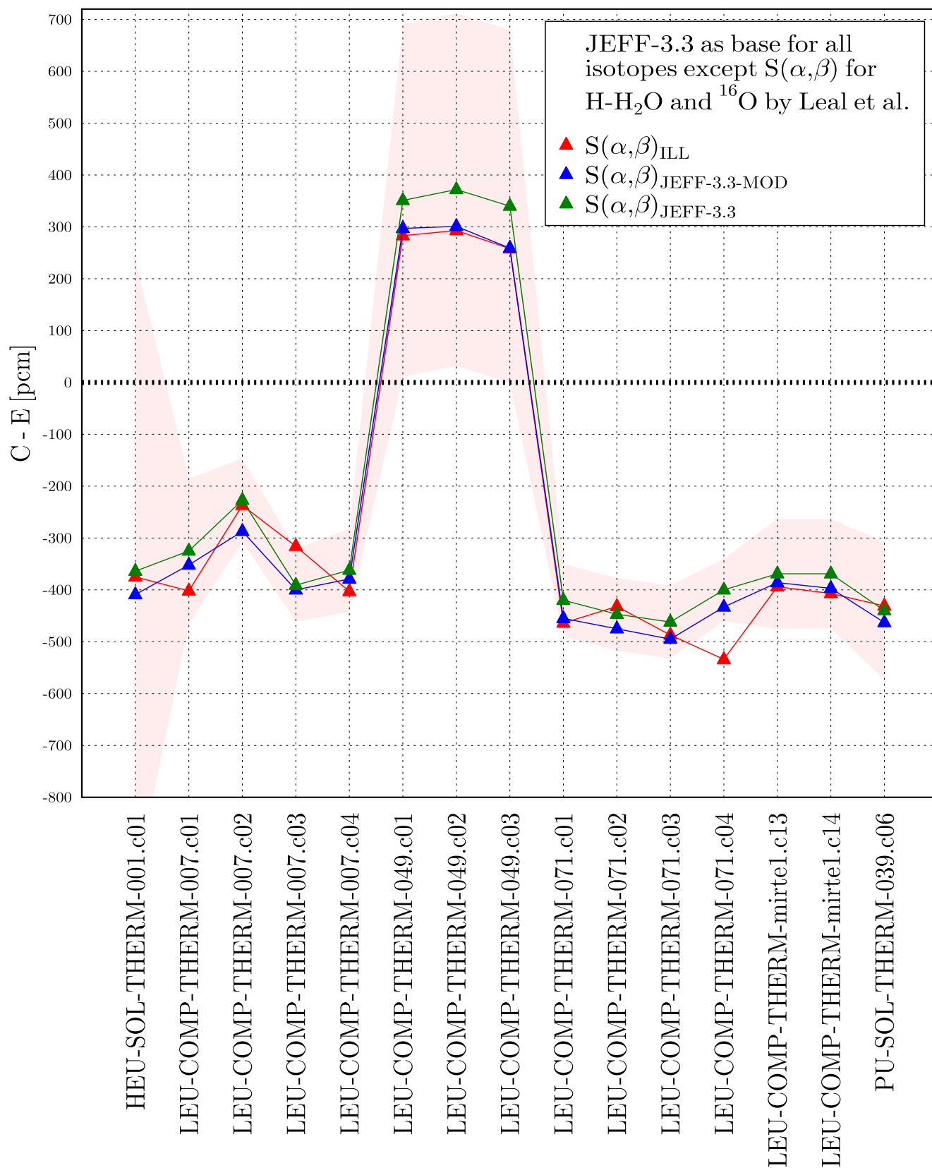
FIGURE 7.13: Calculated - Experimental (C-E) results for the selected ICSBEP benchmark using different TSL evaluations and the IRSN new 16 O evaluation.
