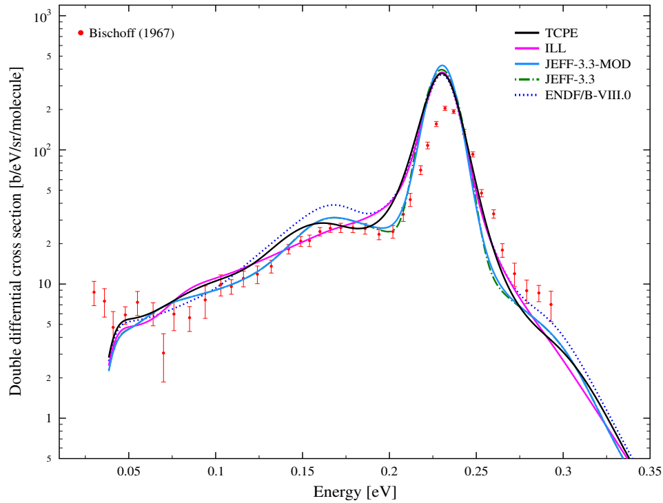
FIGURE 7.4: Double differential scattering cross section of light water at incident energy E = 231 meV and scattering angle \theta=25^\circ .
