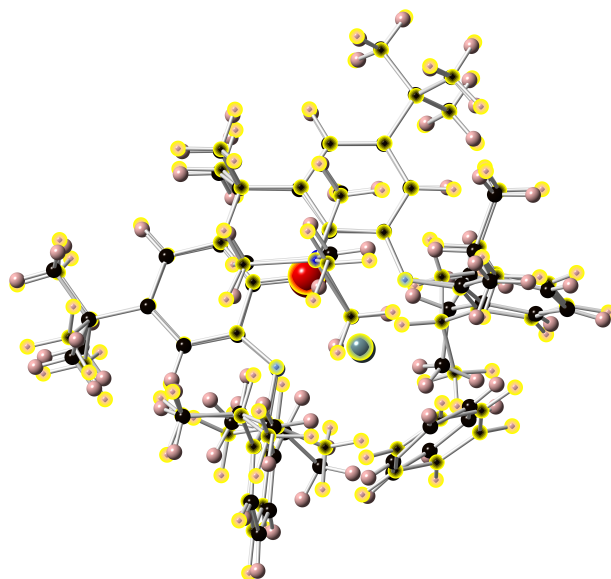
FIGURE 3.14: Superposition of the X-ray and the optimised (yellow atoms) structures of \eta^6\text{-2-U}
