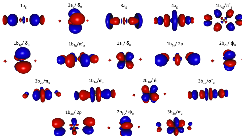
FIGURE 4.6: Molecular orbitals of \text{PuO}_2 at the CASSCF level; Isosurface = 0.05 a.u.
