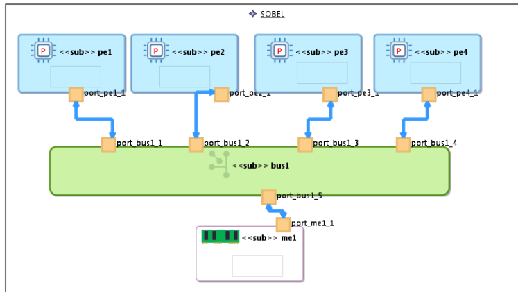
Figure 5.2: platform template for the case study-1 is composed of 6 subsystems: 4 subPE s (in blue), 1 subCommunication (in green), and 1 subMemory (in white)
