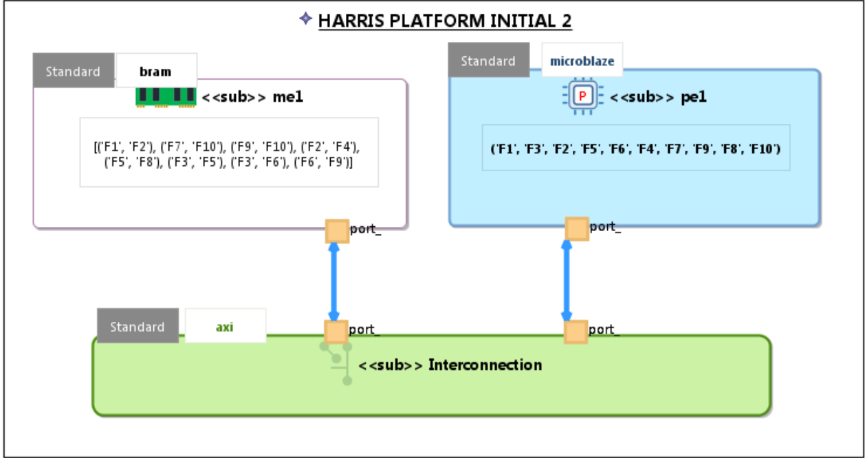
Figure 5.8: initial solution in which all functions are mapped into a single processor, "INITIAL 2", ( R_{platf} = 0.90795063 , T_{sys} = 30.64 ms, C_{platf} = 4.0 ).
