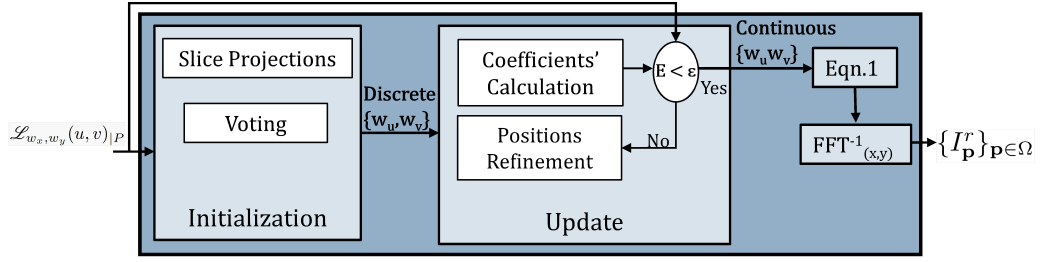
Figure 3.3: An overview of the sparse reconstruction scheme [22].
