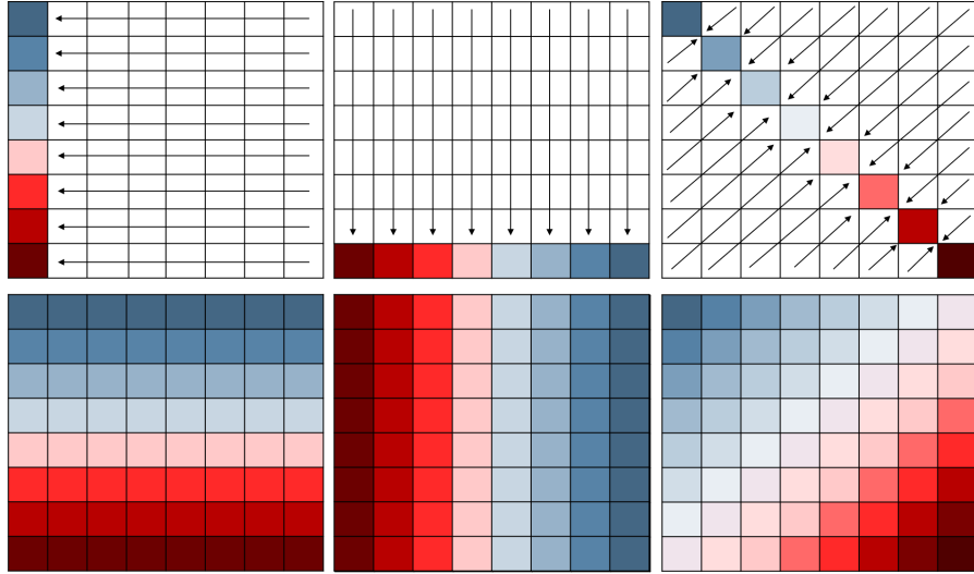
Figure 3.4: Frequency bucketization examples using discrete line Projections. Top: sampled discrete lines. Bottom: projection of the corresponding frequencies.
