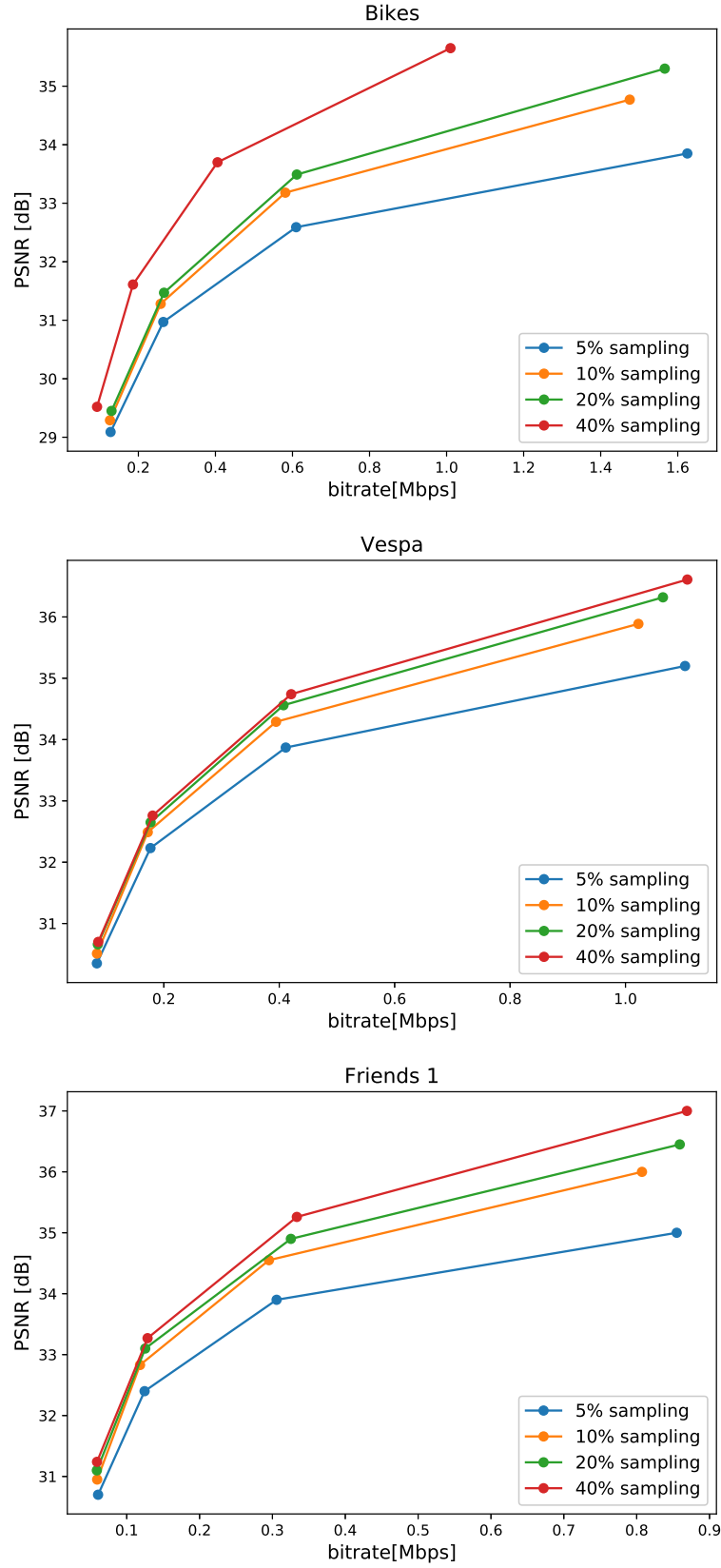
Figure 5.2: Rate-distortion results for plenoptic light fields from the JPEG Pleno Dataset [149].
