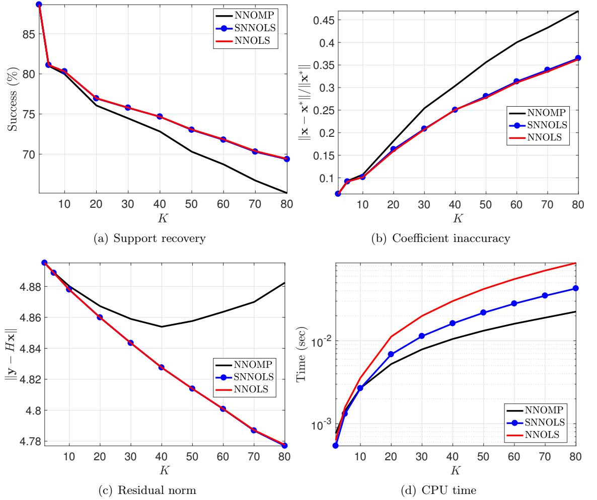
Figure 3.9: Comparison of NNOG algorithms. Performances are averaged over 400 trials in a simulated sparse deconvolution problem with Gaussian kernel with \sigma = 2 , P_n = 10^{-2} , and a dictionary of size 2400 \times 2388 .
