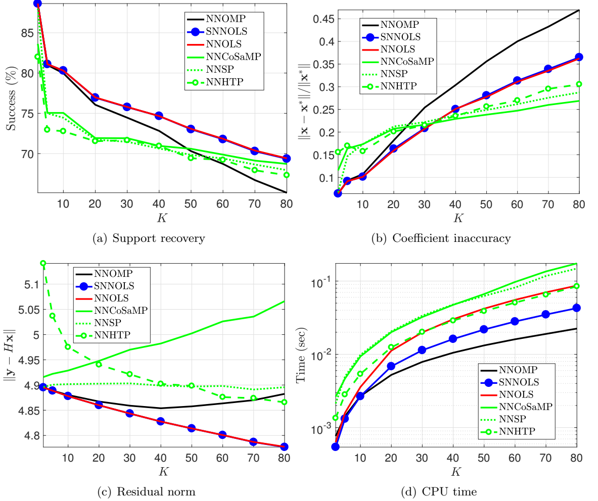
Figure 3.16: Comparison of NNOG algorithms with non-negative versions of CoSaMP, SP, HTP. Performances are averaged over 400 trials in a simulated sparse deconvolution problem with Gaussian kernel with \sigma = 2 , P_n = 10^{-2} , and a dictionary of size 2400 \times 2388 .
