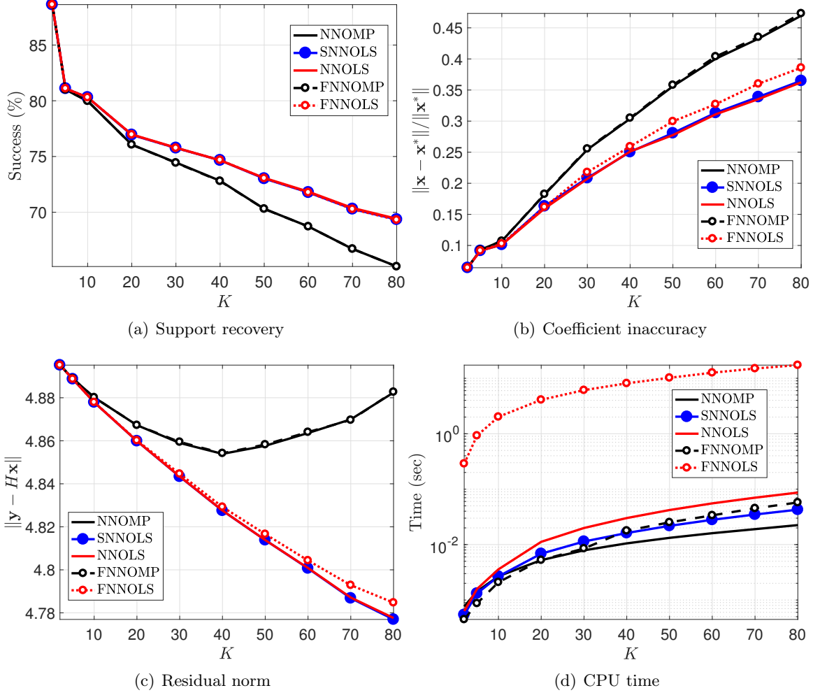
Figure 3.14: Comparison of NNOG algorithms with with approximative fast non-negative greedy algorithms. Performances are averaged over 400 trials in a simulated sparse deconvolution problem with Gaussian kernel with \sigma = 2 , P_n = 10^{-2} , and a dictionary of size 2400 \times 2388 .
