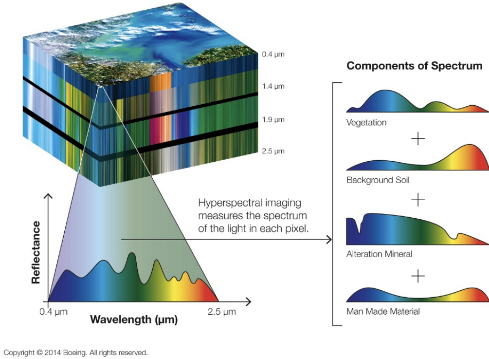
Figure 1.5: Spectral unmixing (image credit: Boeing)
