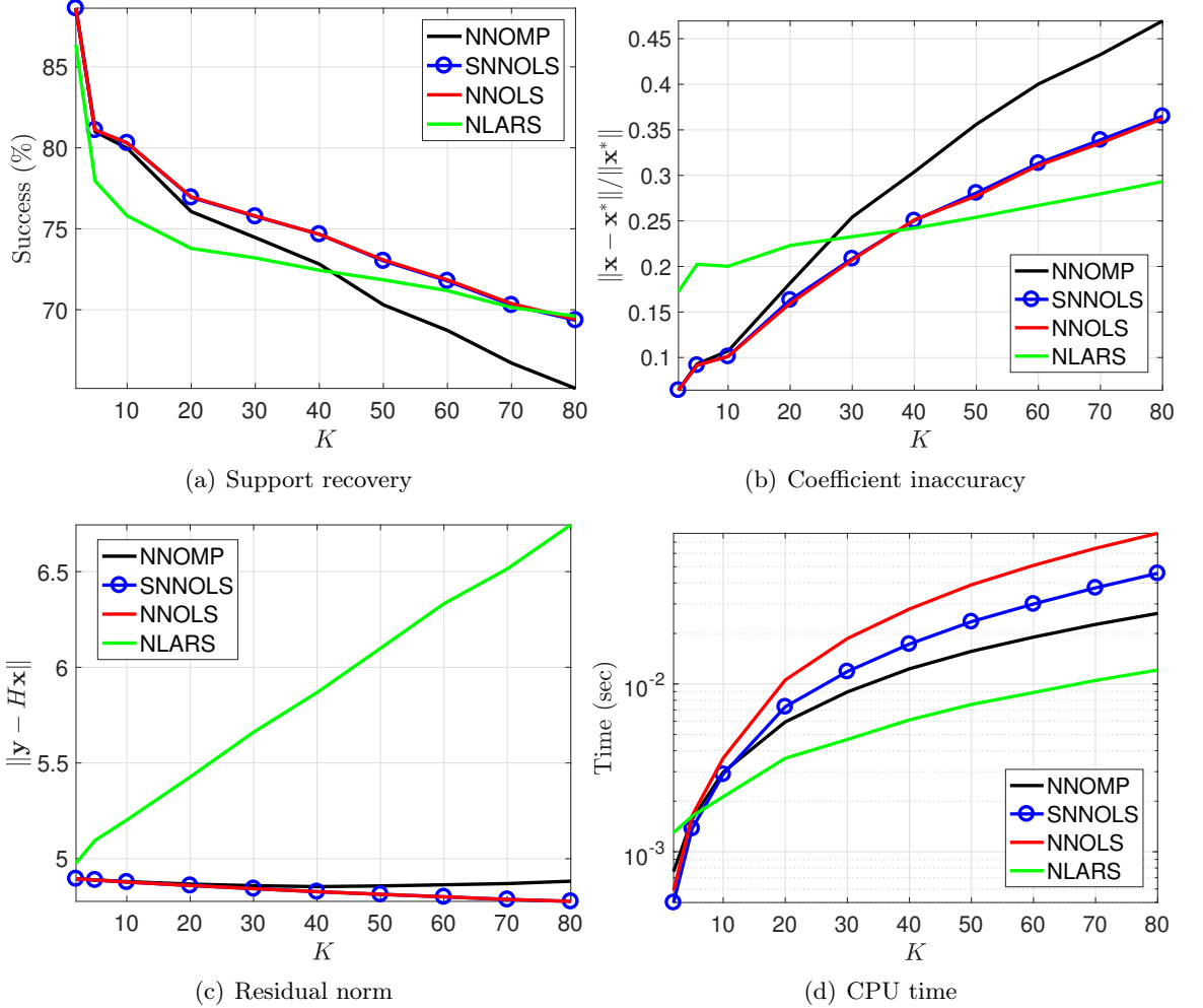
Figure 3.18: Comparison of NNOG algorithms with NLARS. Performances are averaged over 400 trials in a simulated sparse deconvolution problem with Gaussian kernel with \sigma = 2 , P_n = 10^{-2} , and a dictionary of size 2400 \times 2388 .
