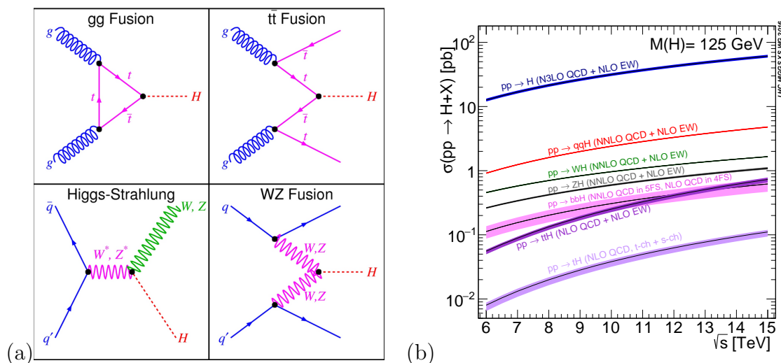
Figure 1.3 – (a) Higgs boson productions modes at LHC: (top left) Gluon-gluon fusion (ggF), (top-right) associated production with a pair of top quarks (ttH), (left-bottom) associated production with a vector boson (WH or ZH) and (right-bottom) vector boson fusion (VBF). (b) Higgs boson production modes cross-sections at LHC in pp \rightarrow H + X processes as a function of \sqrt{s} for a Higgs boson mass m_H = 125 GeV [19].
