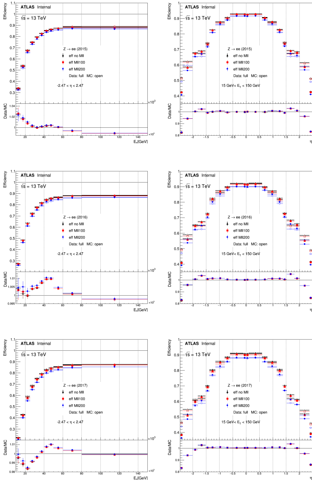
Figure A.14 – Efficiency and SF (ratio) for WP3, WP3 + M(\text{tr}^+, \text{tr}^-) > 100 \text{ MeV} and WP3 + M(\text{tr}^+, \text{tr}^-) > 200 \text{ MeV} in bins of E_T but inclusive in \eta (left) and in bins of \eta but inclusive in E_T (right) for 2015 (top), 2016 (middle) and 2017 (bottom) data.
