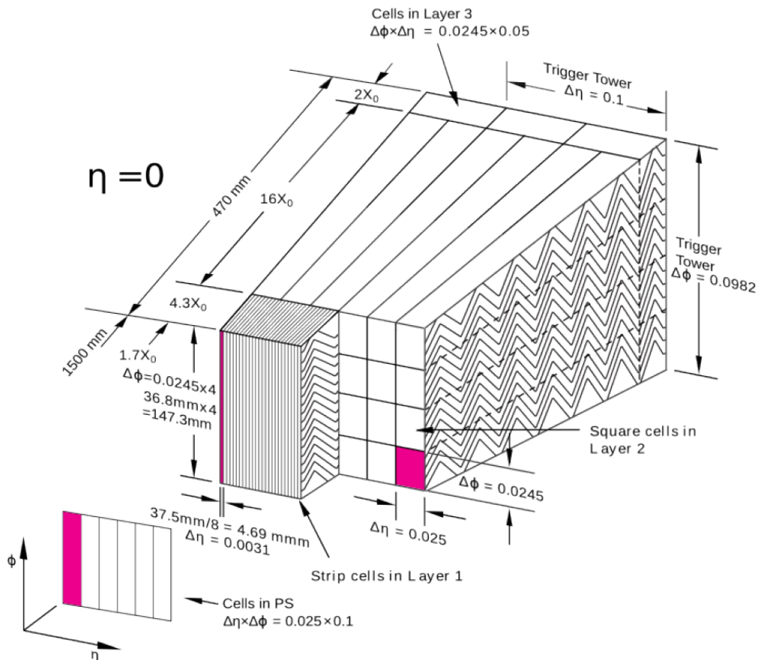
Figure 2.9 – ATLAS detector schematic view: calorimeter system [31].
