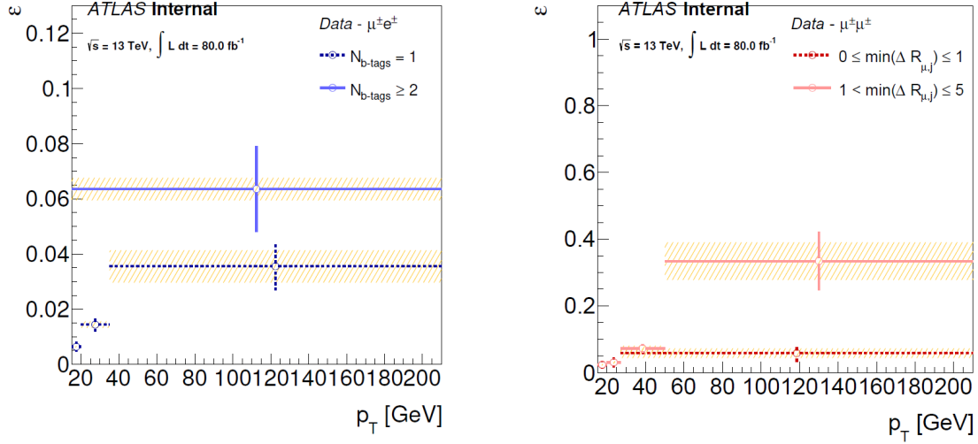
Figure 5.8 – Fake lepton efficiency for electrons (left) and for muons (right) for the 2\ell SS analysis with 80\text{ fb}^{-1} of data at \sqrt{s} = 13\text{ TeV} . The orange band represents the systematic uncertainty on the fake rate.
