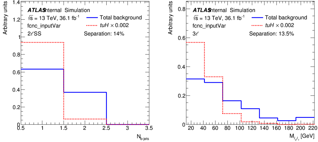
Figure 4.11 – Normalized distribution of the most discriminant variable for t \rightarrow H u signal and all background : Number of b -jet in 2\ell SS pre-MVA region (left) and \ell_0 - \ell_1 invariant mass (right). The first and last bins include the underflows and overflows.
