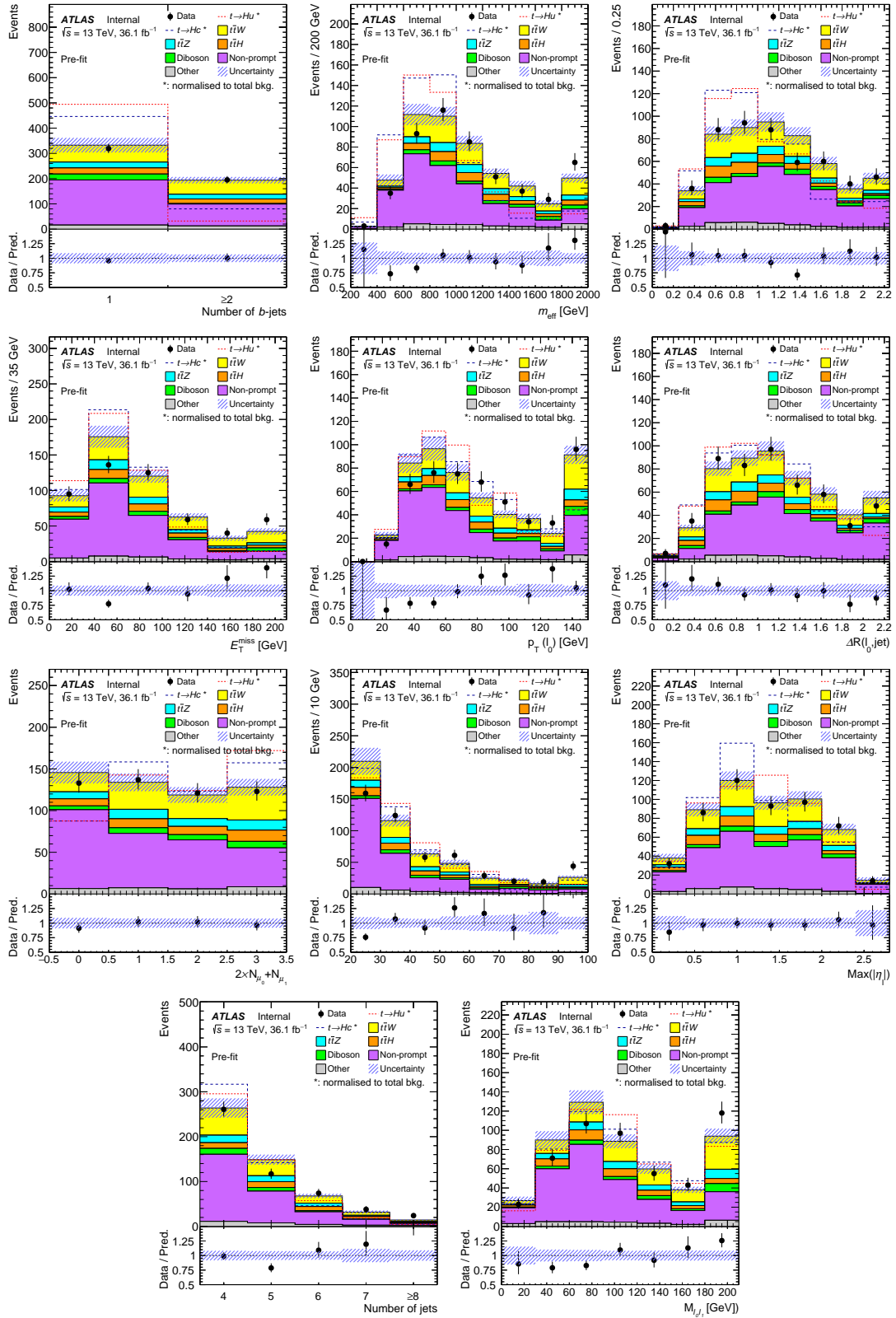
Figure 4.12 – Input variables for 2\ell SS category sorted by separation power. The red dotted (blue dashed) line shows the t \rightarrow Hu^* ( t \rightarrow Hc^* ) shape normalized to the background. The errors for the prediction correspond to statistical and systematic uncertainties. The errors assigned to data are Poissonian.
