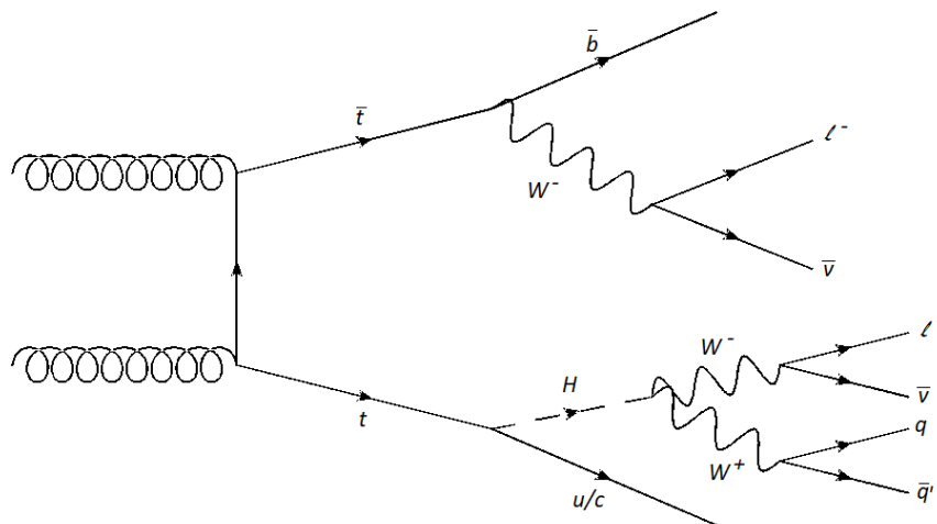
Figure 4.4 – Full decay chain for the t \rightarrow Hq in t\bar{t} processes for 2\ell SS channel.
