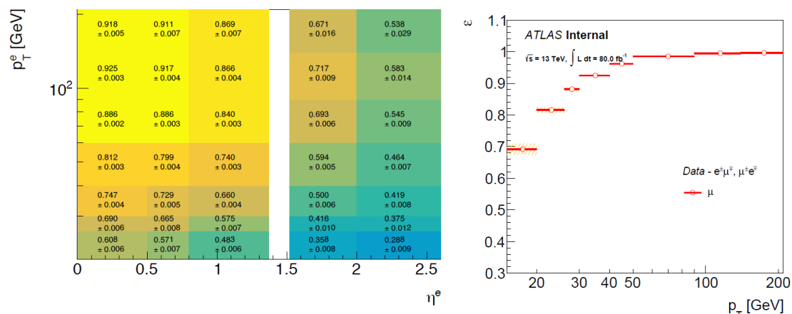
Figure 5.7 – Real efficiency for electrons (left) parametrized in p_T and |\eta| and real efficiency for muons (right) for the 2\ell SS analysis with 80 \text{ fb}^{-1} of data at \sqrt{s} = 13 \text{ TeV} .
