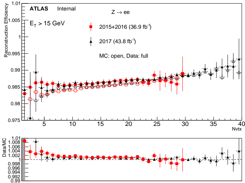
Figure 3.11 – Electron reconstruction efficiency and scale factor dependency on N_{\text{vtx}} .
