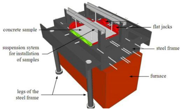
a) Furnace and frame for mechanical loading
