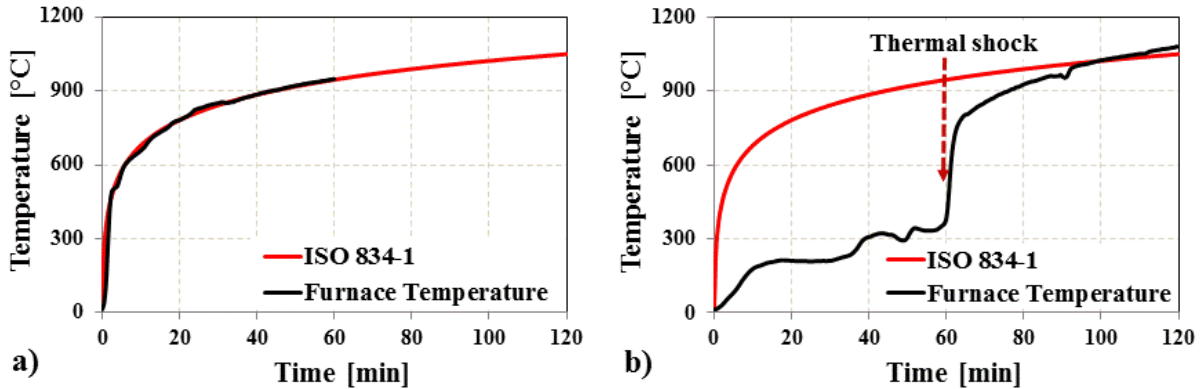
Figure 4.6: Evolution of furnace temperature during ISO 834-1 fire (a) and slow heating with thermal shock (b) test.
