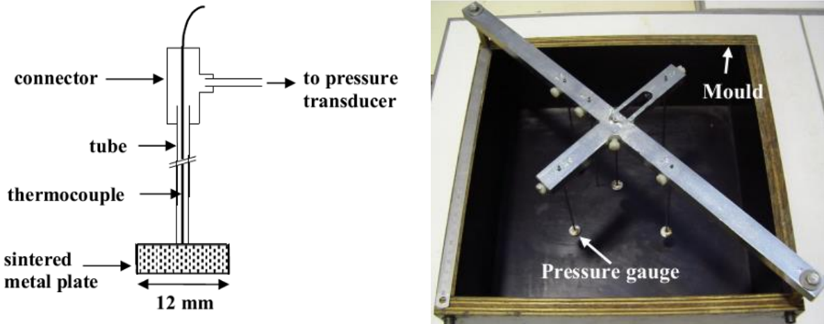
Figure 3.13: Pressure–temperature gauge
