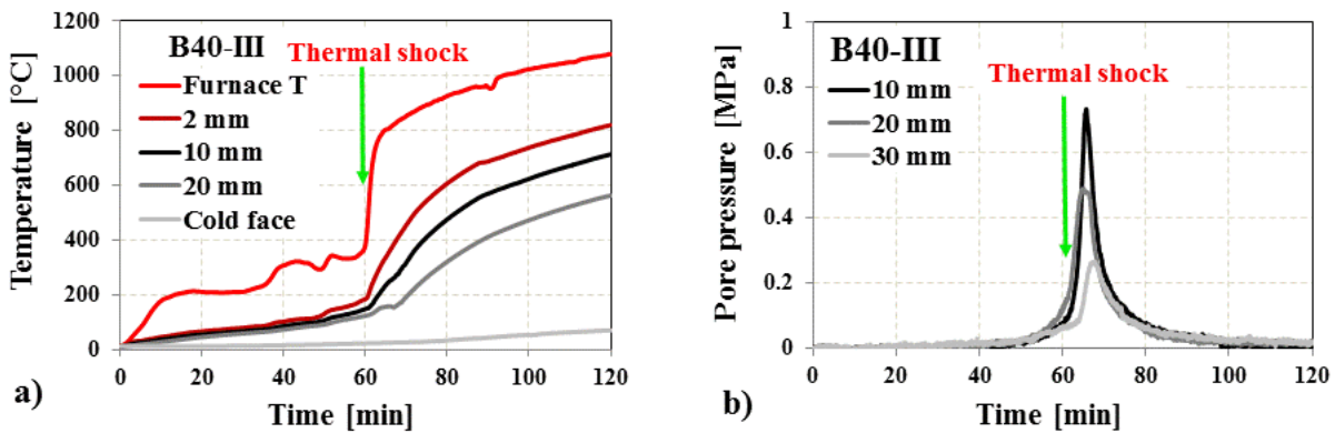
Figure 4.18: Development of temperature (a) and pore pressure (b) inside B40-III concrete during slow heating and thermal shock test.
