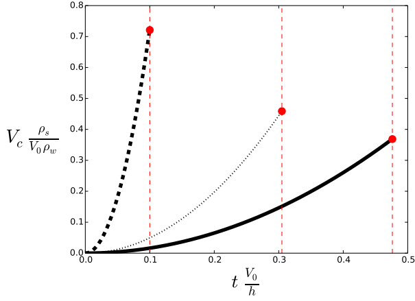
Fig. 5 Caisson sliding velocity for the ideal case (no friction, no uplift) – (–) \alpha = 45^\circ ; (··) \alpha = 60^\circ ; (—) \alpha = 80^\circ
