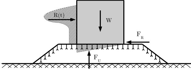
Fig. 2 Forces considered during impact
