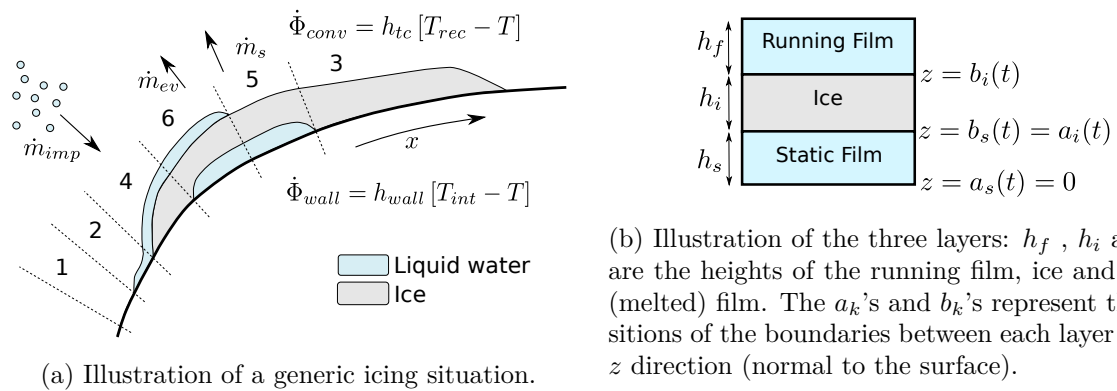
Figure 6.2: Three-layer model in MiLeS2D. Reprinted from [4].
