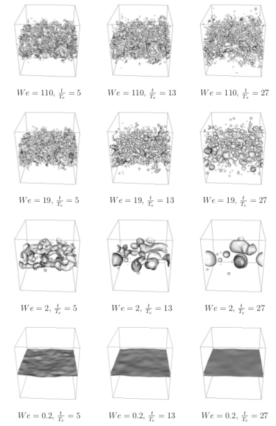
(a) Liquid sheet in a HIT flow for four different W_e numbers at different times t/T_e .
