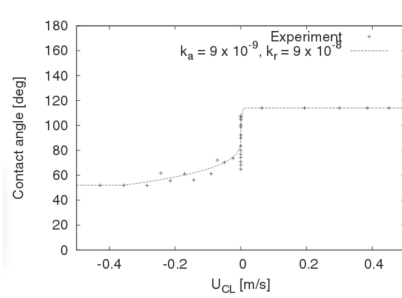
(a) Dynamical contact angle law from Yokoi et al. [44].
