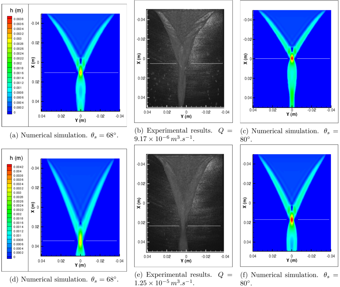
Figure 7.7: Thickness profile at t = 0.3 \text{ s} of a liquid water film injected on a vertical flat plate as a function of the volume flow rate Q . The static contact angle \theta_s is measured experimentally and estimated between 60^\circ and 80^\circ . h_* is chosen so that h_*/h^{bulk} \approx 1/18 . The pinching length is symbolized by the white solid line. Reprinted from [1].
