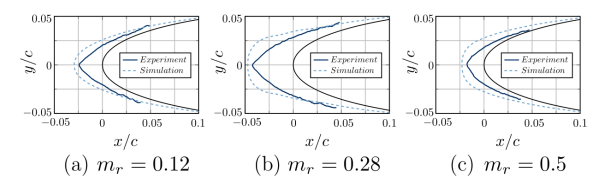
(d) NACA 0012: Simulation versus experiment - side view ice accretion after 120 seconds of icing at T_\infty = 0^\circ C , TWC = 12g/m^3 for a) and b) and TWC = 6.4 g/m^3 for c). Variation of the liquid water ratio LWR .
