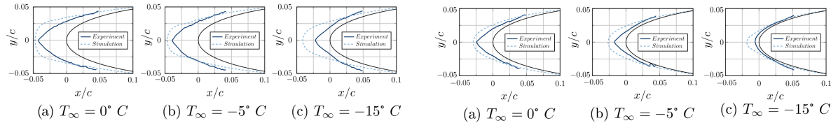
(a) NACA 0012: Simulation versus experiment - side view ice accretion after 120 seconds of icing at TWC = 12 g/m^3 and LWR = 0.28 . Variation of temperature.
