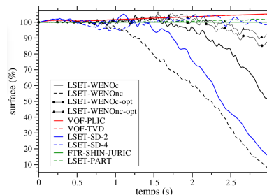
(c) Bell et al. test case [27]. 64^2 grid. Time evolution of the mass of the initial circle for different interface capturing methods. Acronyms are available in [1].
