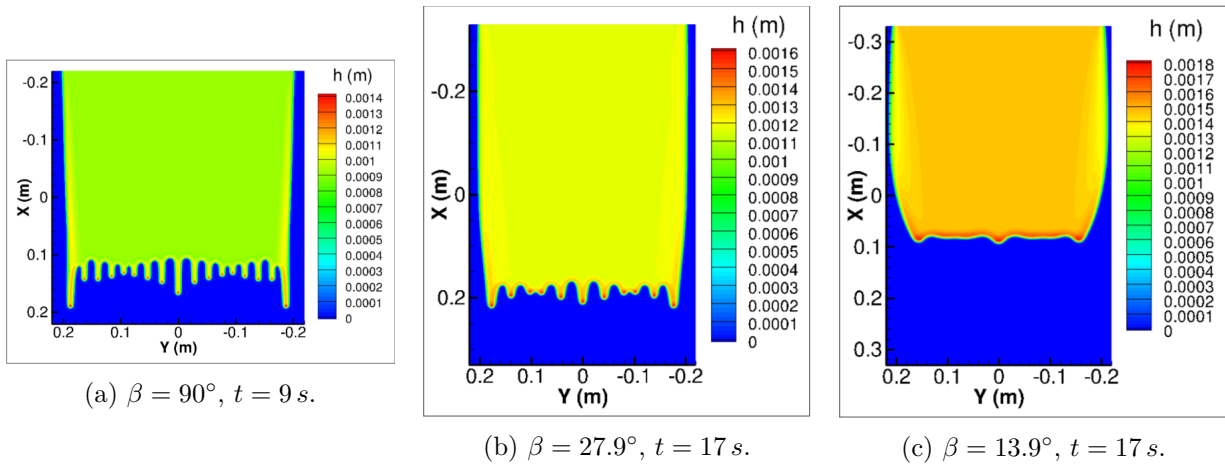
Figure 7.8: Numerical simulations based on Johnson’s experiments [23]. Re = 0.52 . The configurations are summarized in [1]. Reprinted from [1].
