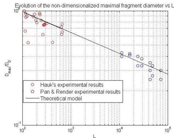
(c) Evolution of the diameter of the biggest fragment vs. the impact parameter \mathcal{L} . Comparison between ONERA fit (solid line) [9], T. Hauk (AGI) experimental results (red circles) [30] and Pan & Render [35] experimental results (blue circles).
