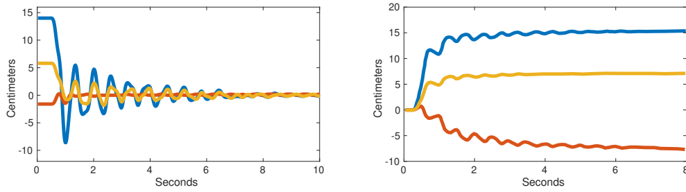
Figure 3.9: Open-loop arm experiment Left: starting from an actuated and deformed state going towards a straight, down-hanging arm position. Right: starting from a straight, down-hanging arm pose going towards a deformed state through an open-loop step actuation. The graph shows the x (red), y (blue) and z (yellow) positions of the arm's end-effector as it is swinging back and forth while asymptotically nearing a straight arm position.
