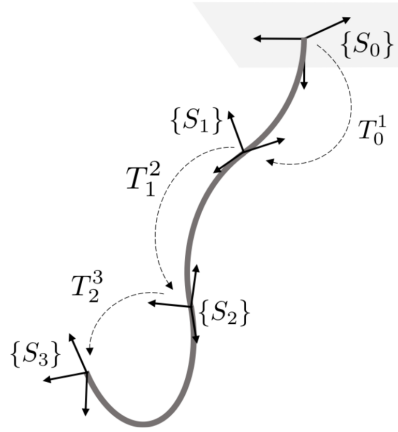
Figure 2.3: Example of 3D piece-wise constant curvature robot composed by 3 sections from Katzschmann, Della Santina, Toshimitsu, Bicchi & Rus (2019).
