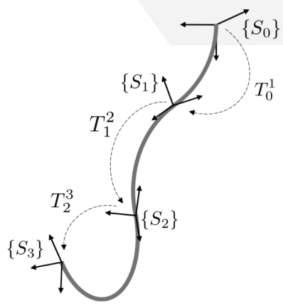
Figure 2.3: Example of 3D piece-wise constant curvature robot composed by 3 sections from (Katzschnann, Della Santina, Toshimitsu, Bicchi & Rus 2019).
