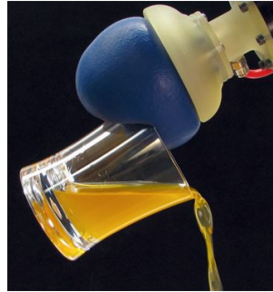
Figure 1.5: Universal soft gripper presented in (Brown et al. 2010).
