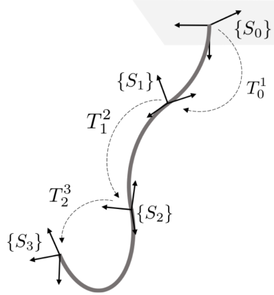
Figure 2.3: Example of 3D piece-wise constant curvature robot composed by 3 sections from (Katschmann, Della Santina, Toshimitsu, Bicchi & Rus 2019).
