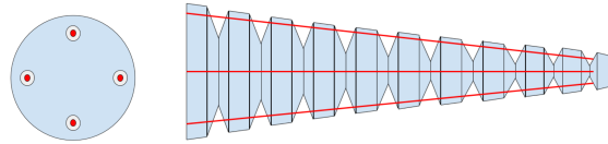
Figure 3.2: Design of the robot: slice view (left) and side view (right). The robot is actuated with 4 cables in red.
