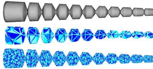
Figure 2.10: Examples of spatial discretization for structure of the trunk robot presented in figure of 3.1; Top: Visual model; Center: Coarse mesh; Bottom: medium-size mesh used in this work.
