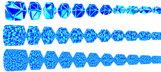
Figure 3.3: Comparison of different FEM mesh of the Trunk-like robot with different accuracy.
