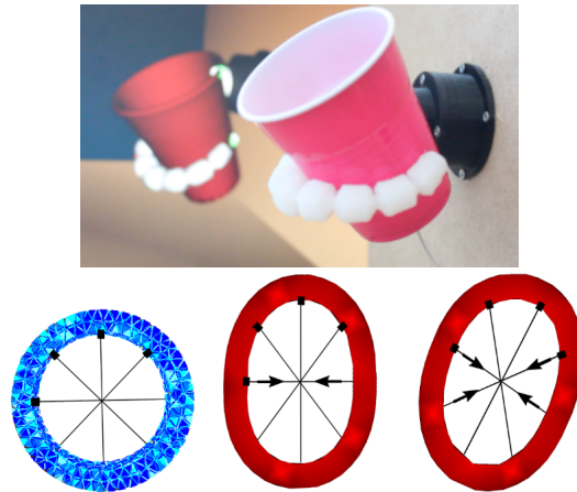
Figure 2.6: Examples of soft robots controlled via a real-time inverse problem based on FEM model, from (Coevoet et al. 2019).
