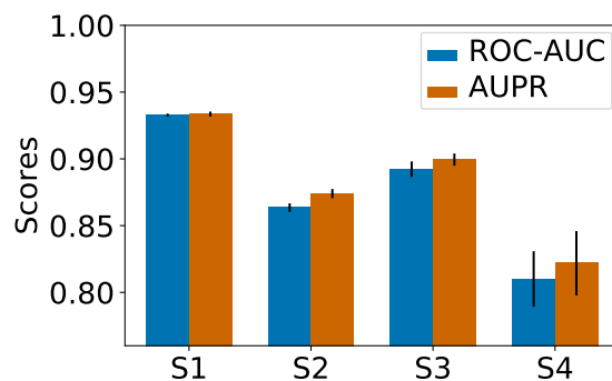
Figure B.1: Nested 5-fold cross-validated area under the ROC curve (ROC-AUC) and area under the precision-recall curve (AUPR) of a multitask SVM on the S_1 - S_4 datasets.
