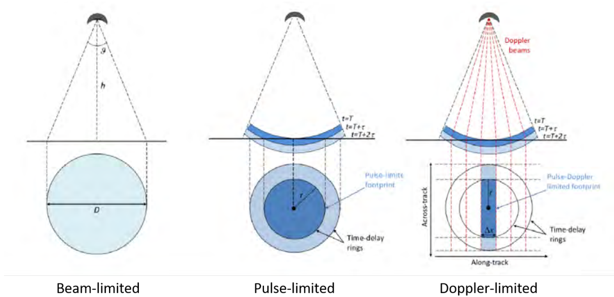
Figure 2.11: Beam-limited, pulse-limited and Doppler-limited altimetry (Sørensen, 2016).
