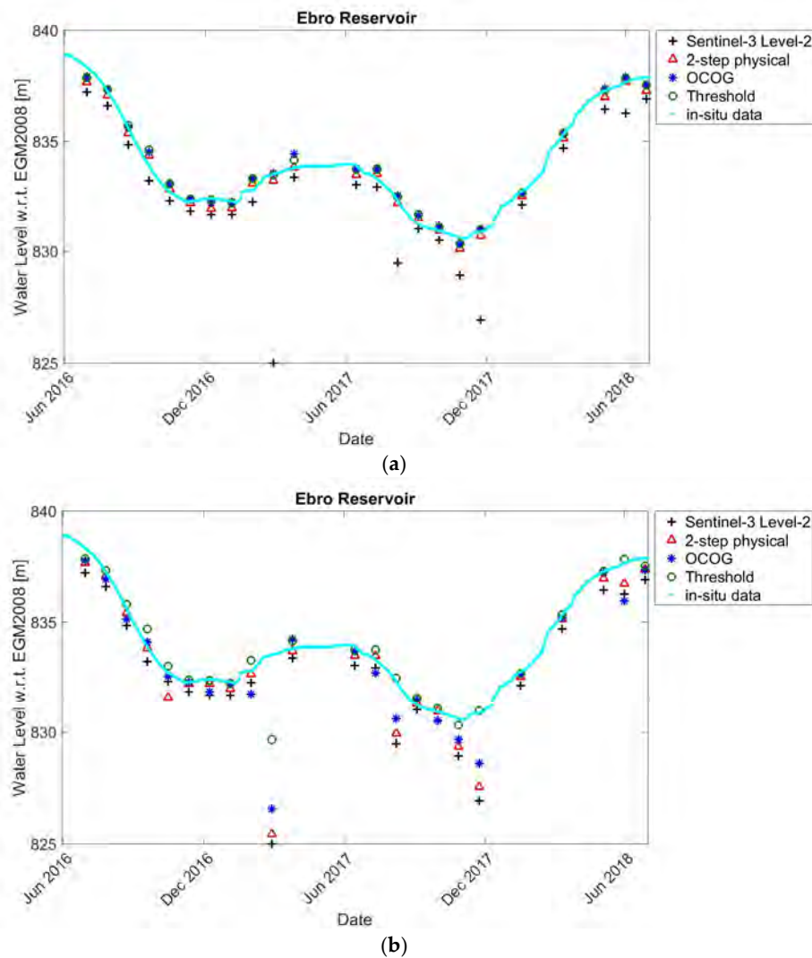
Figure 6. Time series water levels over the Ebro Reservoirs using the waveforms portion selection method (a); and using the whole waveform (b).
