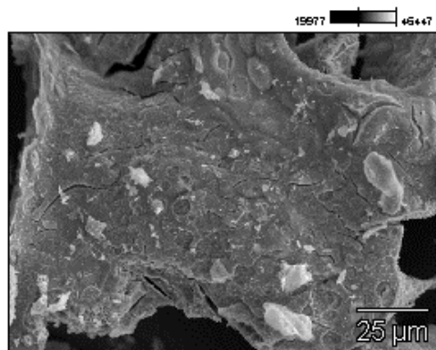
Fig. 5.8(E). SEM image and elemental mapping recorded on \text{La}_{0.6}\text{Ca}_{0.1}\text{Fe}_{0.8}\text{Cu}_{0.2}\text{O}_3 – scale 25\ \mu\text{m} .
