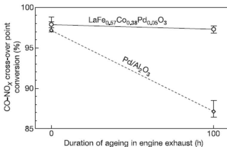
Fig. 2.25. Catalytic activity of \text{LaFe}_{0.57}\text{Co}_{0.38}\text{Pd}_{0.05}\text{O}_3 (Pd-perovskite catalyst) and Pd-impregnated- \text{Al}_2\text{O}_3 (Pd/alumina catalyst) during the ageing process at 900^\circ\text{C} lasting 100h. The conversion efficiency was investigated three times for each sample by the sweep test. The symbol represents the CO-NO x cross-over point conversion (With air-to-fuel ratio \lambda=1 ) and error bars signify corresponding maximum and minimum values. (picture reproduced with permission of Y. Nishihata 2002)
