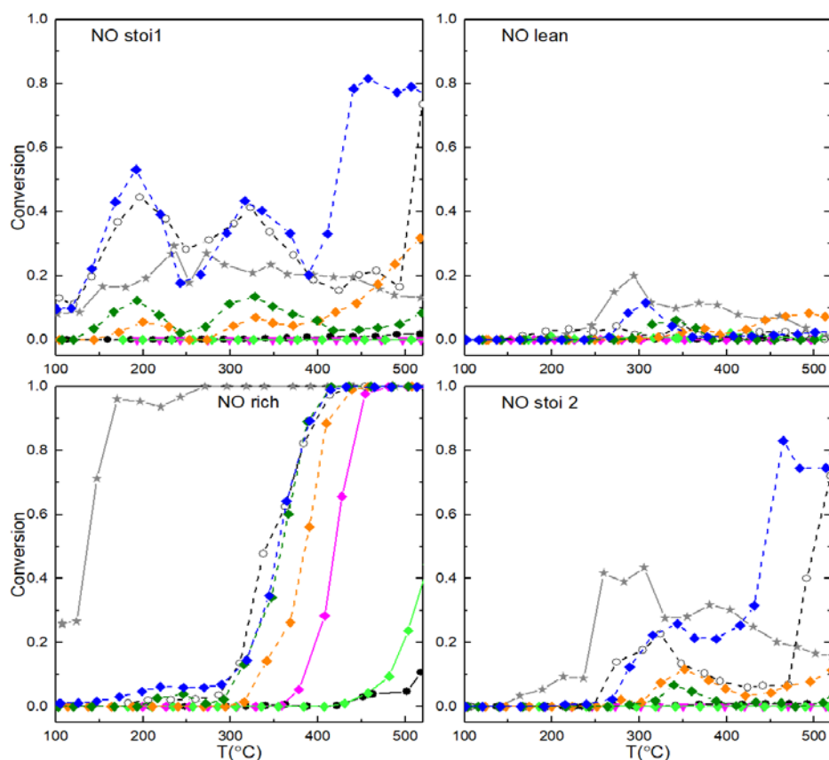
Fig. 7.12. Catalytic reduction performance of iron-based perovskite solid \text{ABO}_3 ( A=\text{La}, \text{Ca} ; B=\text{Fe}, \text{Cu} ) +0.5 wt.%Pd. Grey star solid line ( \star ):commercial reference catalyst; black circle solid line: \text{LaFeO}_3 ( \bullet ); magenta downward triangle solid line: \text{La}_{0.7}\text{Fe}_{0.8}\text{Cu}_{0.2}\text{O}_3 ( \blacktriangledown ); green diamond solid line: \text{La}_{0.6}\text{Ca}_{0.2}\text{Fe}_{0.8}\text{Cu}_{0.2}\text{O}_3 ( \blacklozenge ); blank circle dash line: \text{Pd}/\text{LaFeO}_3 ( \circ );orange diamond dash line: \text{Pd}/\text{La}_{0.6}\text{Ca}_{0.1}\text{Fe}_{0.8}\text{Cu}_{0.2}\text{O}_3 ( \blacklozenge ); olive diamond dash line: \text{Pd}/\text{La}_{0.6}\text{Ca}_{0.2}\text{Fe}_{0.8}\text{Cu}_{0.2}\text{O}_3 ( \blacklozenge ); blue diamond dash line: \text{Pd}/\text{La}_{0.6}\text{Ca}_{0.4}\text{Fe}_{0.8}\text{Cu}_{0.2}\text{O}_3 ( \blacklozenge ).
