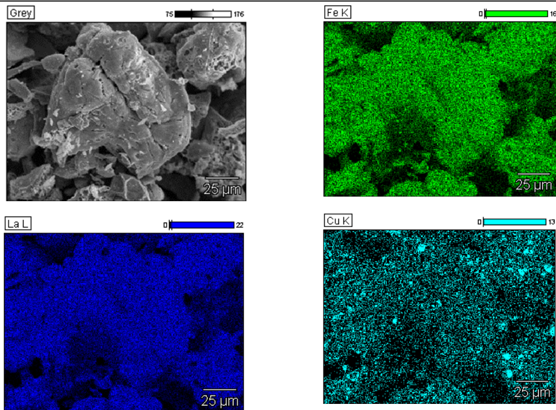
Fig. 5.8(D). SEM image and elemental mapping recorded on \text{La}_{0.7}\text{Fe}_{0.8}\text{Cu}_{0.2}\text{O}_3 – scale 25 \mu\text{m} .
