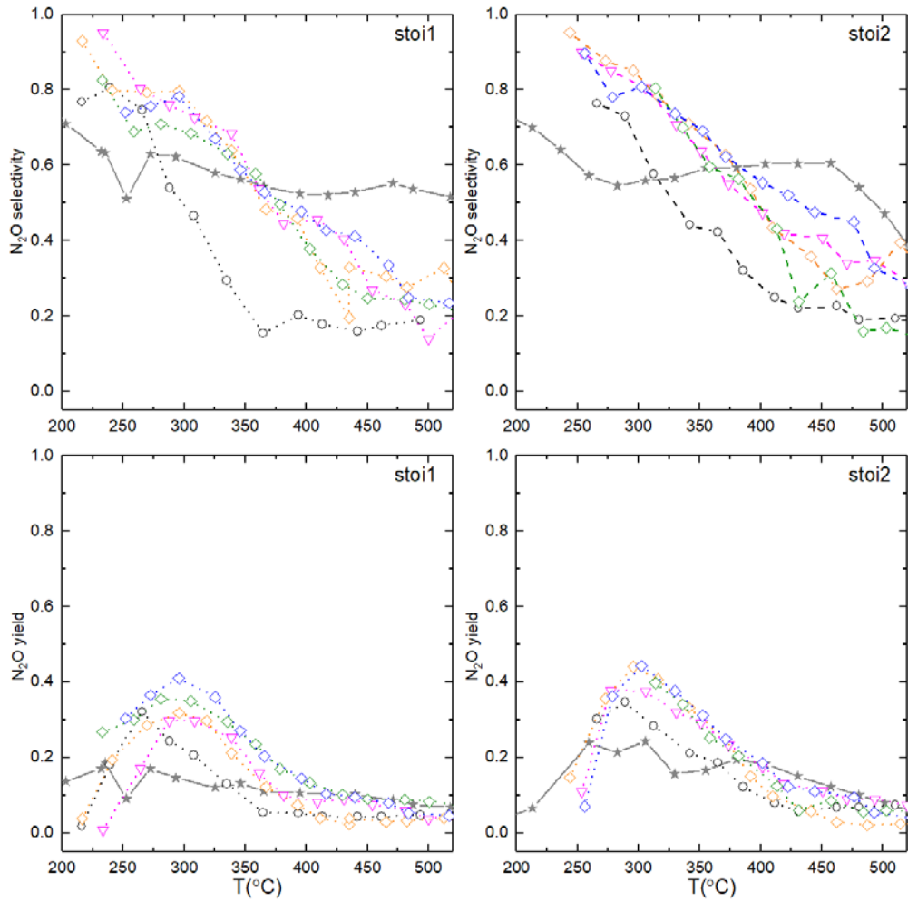
Fig. 8.16. \text{N}_2\text{O} selectivity and yield in stoichiometric atmosphere of iron-based perovskite solid \text{ABO}_3 (A=La, Ca; B= Fe, Cu) +0.1 wt.%Rh. Grey star solid line: commercial reference catalyst(★); black hollow circle dash line: \text{LaFeO}_3+0.1 \text{ wt.\%Rh} (○); magenta downward hollow triangle dash line: \text{La}_{0.7}\text{Fe}_{0.8}\text{Cu}_{0.2}\text{O}_3+0.1 \text{ wt.\%Rh} (▼); orange diamond dash line: \text{La}_{0.6}\text{Ca}_{0.1}\text{Fe}_{0.8}\text{Cu}_{0.2}\text{O}_3+0.1 \text{ wt.\%Rh} (◇); olive diamond dash line: \text{La}_{0.6}\text{Ca}_{0.2}\text{Fe}_{0.8}\text{Cu}_{0.2}\text{O}_3+0.1 \text{ wt.\%Rh} (◇); blue diamond dash line: \text{La}_{0.6}\text{Ca}_{0.4}\text{Fe}_{0.8}\text{Cu}_{0.2}\text{O}_3+0.1 \text{ wt.\%Rh} (◇).
