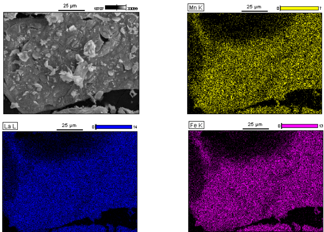
Fig. 6.7(B). SEM image and elemental mapping recorded on \text{La}_{0.7}\text{Fe}_{0.8}\text{Mn}_{0.2}\text{O}_3 . scale:25 \mu\text{m}
