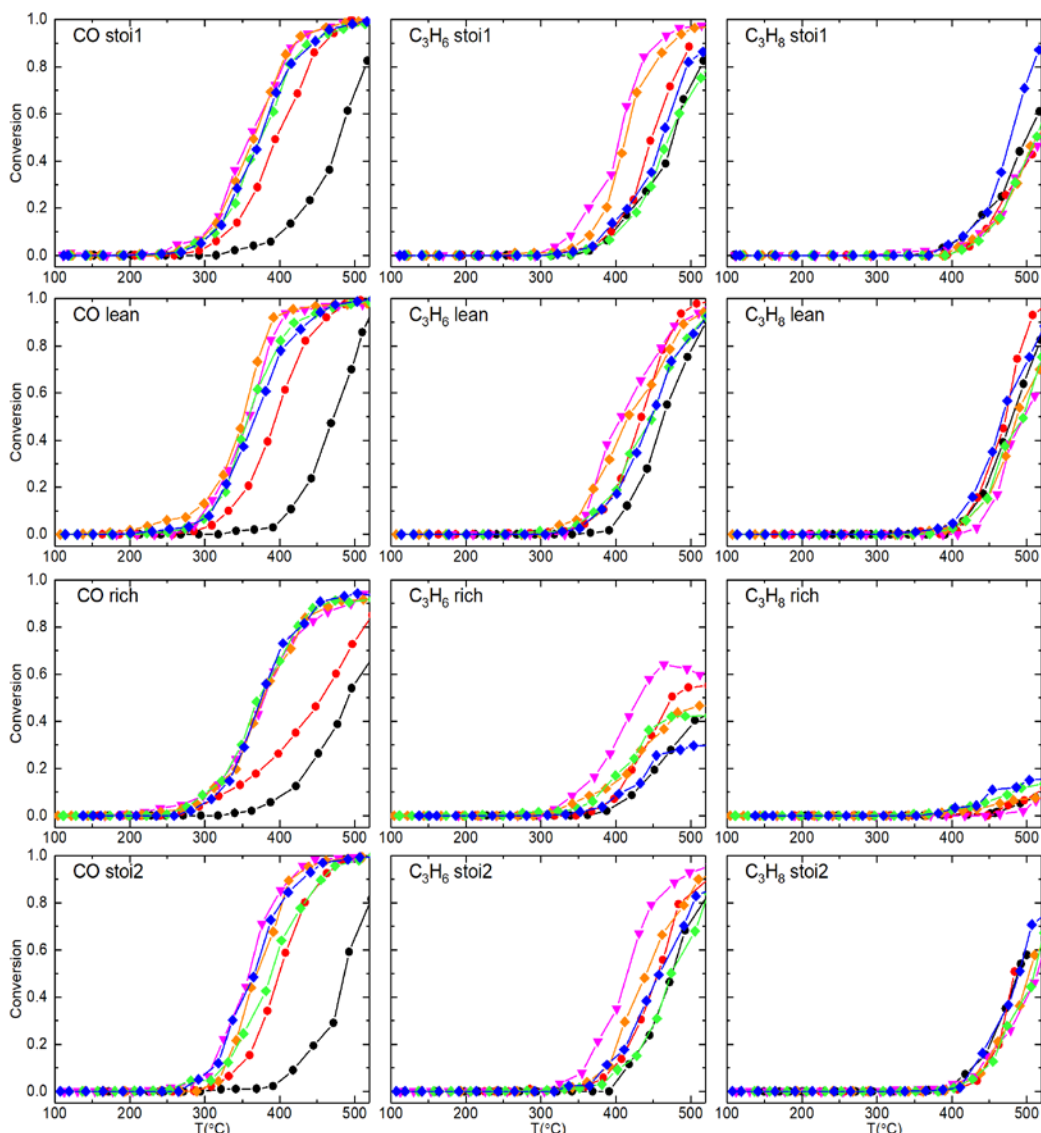
Fig. 6.22. Catalytic oxidation performance of iron-based perovskite solid \text{ABO}_3 doped with calcium and manganese ( A=\text{La}, \text{Ca} ; B=\text{Fe}, \text{Mn} ) black circle: \text{LaFeO}_3 (●); red circle: \text{La}_{0.7}\text{FeO}_3 (●); magenta downward triangle: \text{La}_{0.7}\text{Fe}_{0.8}\text{Mn}_{0.2}\text{O}_3 (▼); orange diamond: \text{La}_{0.6}\text{Ca}_{0.1}\text{Fe}_{0.8}\text{Mn}_{0.2}\text{O}_3 (◆); green diamond: \text{La}_{0.6}\text{Ca}_{0.2}\text{Fe}_{0.8}\text{Mn}_{0.2}\text{O}_3 (◆); blue diamond: \text{La}_{0.6}\text{Ca}_{0.4}\text{Fe}_{0.8}\text{Mn}_{0.2}\text{O}_3 (◆).
