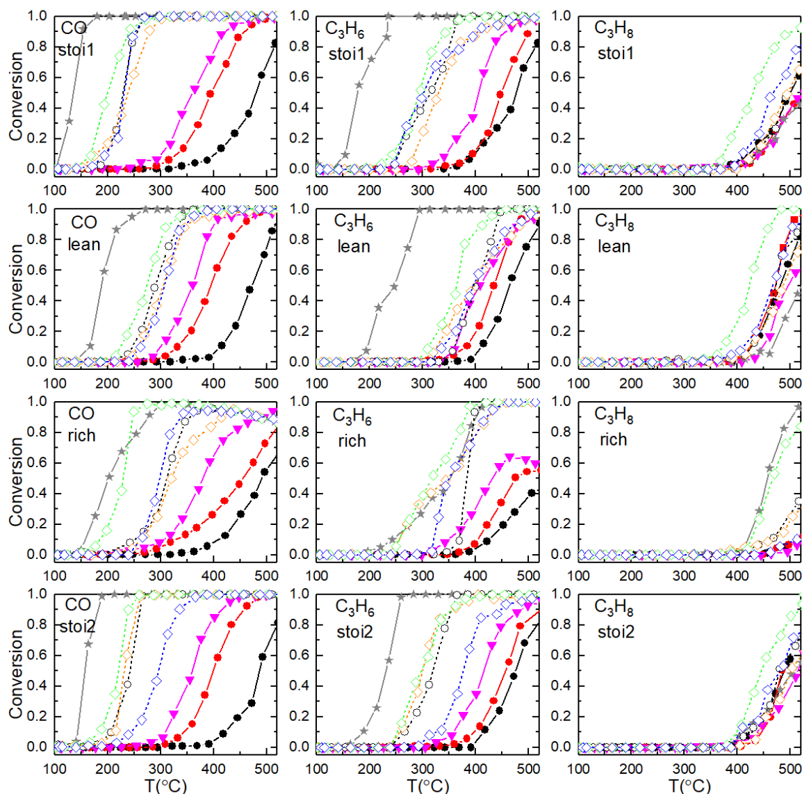
Fig. 9.4. Catalytic oxidation performance of iron-based perovskite solid \text{ABO}_3 ( \text{A}=\text{La}, \text{Ca} ; \text{B}=\text{Fe}, \text{Mn} ) +0.1 \text{ wt.}\% \text{Rh} . Grey star solid line: commercial reference catalyst ( \star ); black circle solid line: \text{LaFeO}_3 ( \bullet ); red circle solid line: \text{La}_{0.7}\text{FeO}_3 ( \bullet ); magenta downward triangle solid line: \text{La}_{0.7}\text{Fe}_{0.8}\text{Mn}_{0.2}\text{O}_3 ( \blacktriangledown ); black hollow circle dash line: \text{LaFeO}_3+0.1 \text{ wt.}\% \text{Rh} ( \circ ); orange diamond dash line: \text{La}_{0.6}\text{Ca}_{0.1}\text{Fe}_{0.8}\text{Mn}_{0.2}\text{O}_3+0.1 \text{ wt.}\% \text{Rh} ( \diamond ); green diamond dash line: \text{La}_{0.6}\text{Ca}_{0.2}\text{Fe}_{0.8}\text{Mn}_{0.2}\text{O}_3+0.1 \text{ wt.}\% \text{Rh} ( \diamond ); blue diamond dash line: \text{La}_{0.6}\text{Ca}_{0.4}\text{Fe}_{0.8}\text{Mn}_{0.2}\text{O}_3+0.1 \text{ wt.}\% \text{Rh} ( \diamond ).
