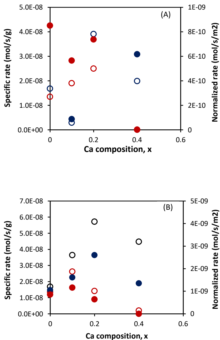
Fig. 9.9. Comparison of specific and normalized rates for propene oxidation measured at 375°C on Rh/La 0.6 Ca x Fe 0.8 Cu 0.2 O 3 (A); at 250 °C on Rh/La 0.6 Ca x Fe 0.8 Mn 0.2 O 3 (B) : ○ specific rate (STO1); ○ specific rate (STO2); ● normalized rate (STO1); ● Normalized rate (STO2).
