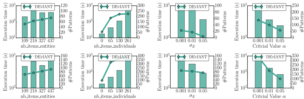
Figure 4.9: Effectiveness of DEVIANT on EPD8 when varying sizes of both description spaces \mathcal{D}_E and \mathcal{D}_I , minimum context support threshold \sigma_E and the critical value \alpha . Default parameters: full description spaces \mathcal{D}_E and \mathcal{D}_I , \sigma_E = 0.1\% , \sigma_I = 1\% and \alpha = 0.05 . Bootstrapping Confidence intervals for handling variability of outcomes is disabled in the figures on the top row, and enabled in the figures on the bottom row.
