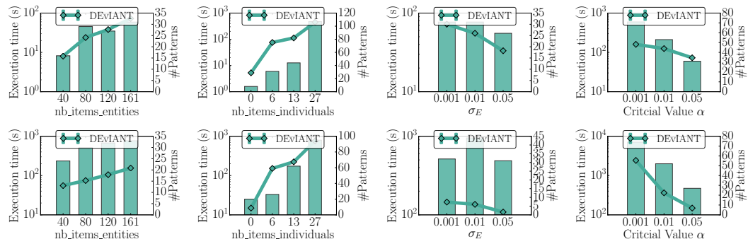
Figure 4.11: Effectiveness of DEVIANT on Movielens when varying sizes of both description spaces \mathcal{D}_E and \mathcal{D}_I , minimum context support threshold \sigma_E and the critical value \alpha . Default parameters: full description spaces \mathcal{D}_E and \mathcal{D}_I , \sigma_E = 0.1\% , \sigma_I = 1\% and \alpha = 0.05 . Bootstrapping Confidence intervals for handling variability of outcomes is disabled in the figures on the top row, and enabled in the figures on the bottom row.
