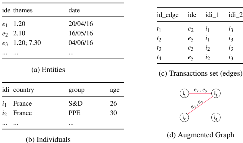
Figure A.1: Example of input data format for Cosmic after transforming the behavioral dataset given in Table 3.1 to an augmented graph and its corresponding transactions set according to the observed discords.
