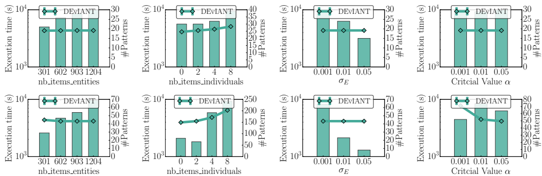
Figure 4.12: Effectiveness of DEVIANT on Yelp when varying sizes of both description spaces \mathcal{D}_E and \mathcal{D}_I , minimum context support threshold \sigma_E and the critical value \alpha . Default parameters: full description spaces \mathcal{D}_E and \mathcal{D}_I , \sigma_E = 0.1\% , \sigma_I = 1\% and \alpha = 0.05 . Bootstrapping Confidence intervals for handling variability of outcomes is disabled in the figures on the top row, and enabled in the figures on the bottom row.
