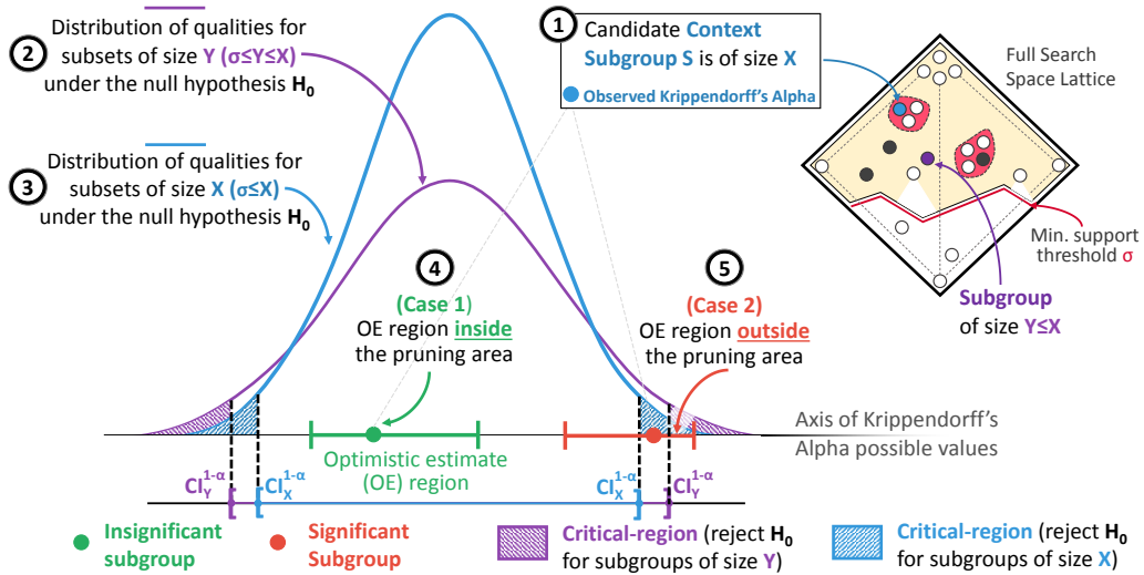
Figure 4.2: Main DEVIANT properties for safe sub-search space pruning. A subgroup is reported as significant if its related Krippendorff's Alpha falls in the critical region of the corresponding empirical distribution of random subsets (DFD). When traversing the search space downward (decreasing support size), the approximate confidence intervals are nested. If the optimistic estimates region falls into the confidence interval computed on the related DFD, the sub-search space can be safely pruned.
