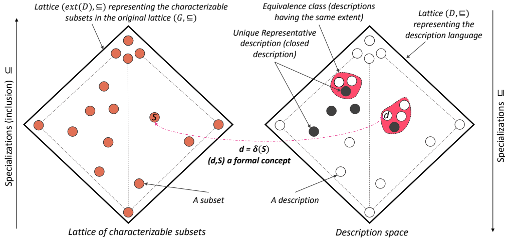
Figure 2.3: Pattern structure (G, (\mathcal{D}, \sqsubseteq), \delta) represented by its associated description language (\mathcal{D}, \sqsubseteq) and the collection of characterizable subsets of the powerset 2^G . Note that, the collection of characterizable subsets \text{ext}[\mathcal{D}] with the inclusion form a lattice. Also, the derivation operators \text{ext} and \delta are order reversing, i.e. d \sqsubseteq d' \Rightarrow G^d \subseteq G^{d'} and F \subseteq F' \Rightarrow \delta(F') \sqsubseteq \delta(F) .
