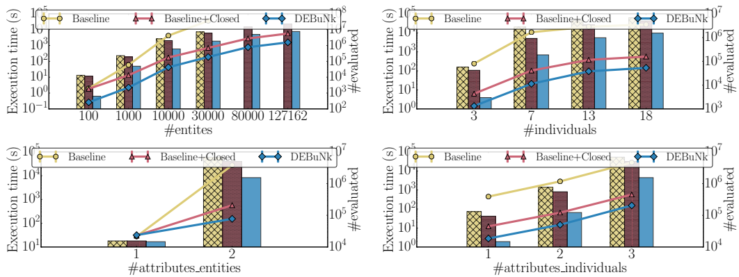
Figure 3.13: Effectiveness of DEBuNk considering Yelp Dataset with |G_E| = 25000 , |G_I| = 18 , |Outcomes| = 146k , |\mathcal{A}_E| = 2 , |\mathcal{A}_I| = 3 , \sigma_E = 5 , \sigma_I = 1 , \sigma_\varphi = 0.5 and \varphi_{dissent} . Lines correspond to the execution time and bars correspond to the number of evaluated patterns.
