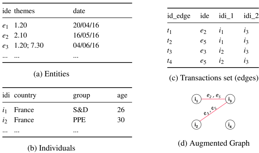
Figure A.1: Example of input data format for Cosmic after transforming the behavioral dataset given in Table 3.1 to an augmented graph and its corresponding transactions set according to the observed discords.
