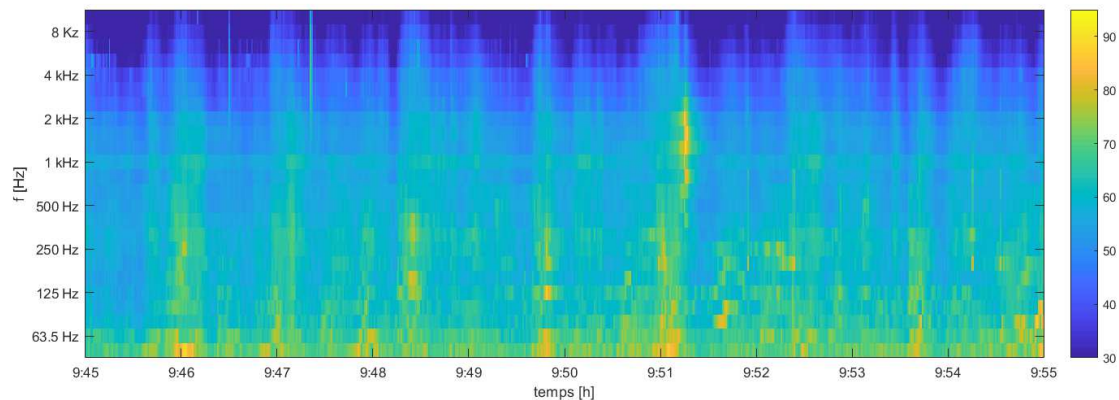
Figure 1:7 Evolution of the L_{eq,f,1s} by octave band f , at a measurement point of Paris XIII , (69 boulevard Auguste Blanqui), over a period of 10 mn (day of March 2, 2015, period [9:45-9:55]). Source of measurements: Lavandier et al. (2017) .
