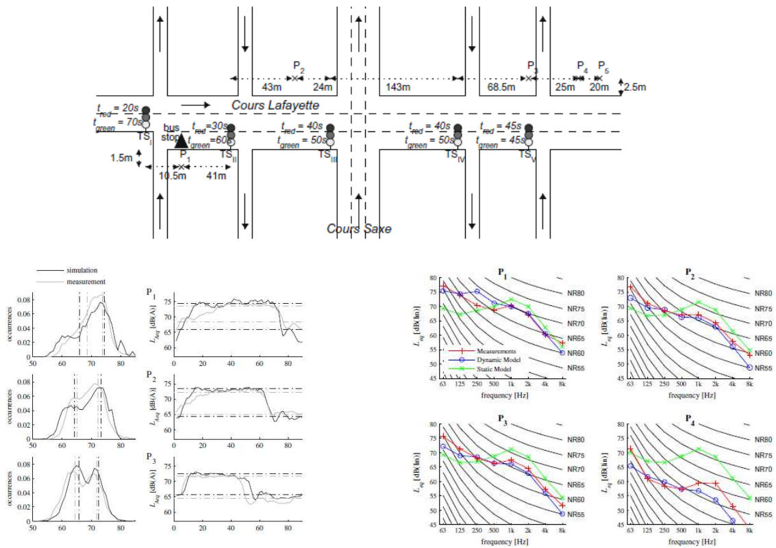
Figure 3:11. Validation of dynamic noise coupling performed by Ifsttar. Top: network implemented in Can et al. (2009b) . Bottom left: extracts from L_{Aeq,1s} distributions. Bottom right: measured and simulated NR curves. Sources: Can et al. (2009b) , Can et al. (2010b) .
