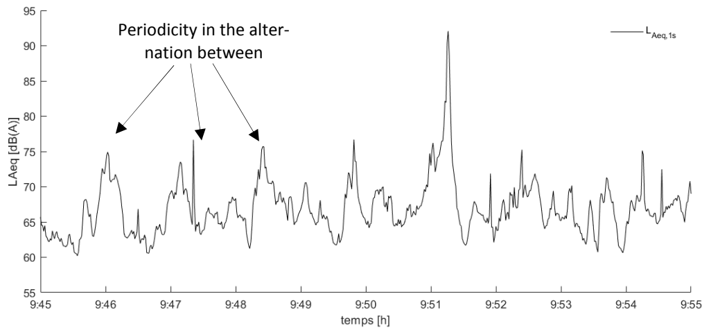
Figure 1:6 Evolution of the L_{Aeq,1s} at a Paris XIII measurement point, over a period of 10 mn (69 boulevard Auguste Blanqui, day of March 2, 2015, period [9:45-9:55]). Source of measurements: Lavandier et al. (2017) .
