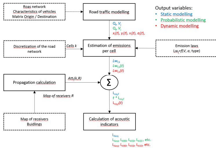
Figure 3:3 Generic scheme of physical models for estimating road traffic noise
