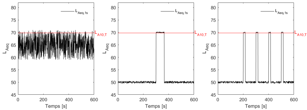
Figure 1:10 Three different L_{Aeq,1s} time series for the same L_{A10,T} .
