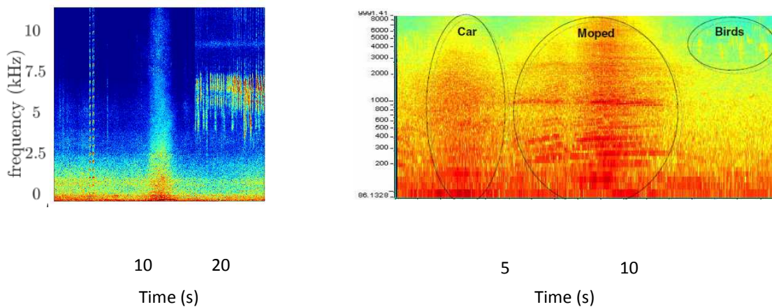
Figure 1:17 Example of spectrograms composed of several sources. Left: spectrogram composed of a vehicle passing noise, a horn, and a bird whistle (Source: Gloaguen et al., 2018 ). Right: spectrogram composed of a vehicle, a moped and birds (Defréville, 2006).
