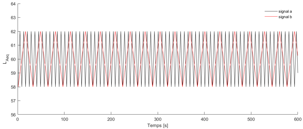
Figure 1:12 Two time series with the same \sigma_{L_{Aeq}} but a different \overline{\delta_{L_{Aeq},1s}} .
