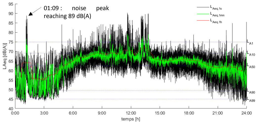
Figure 1:4 Evolution of the L_{Aeq,1s} at a Paris XIII measurement point, over a period of 24-hours (69 boulevard Auguste Blanqui, day of March 2, 2015). Source of measurements: Lavandier et al. (2017) .
