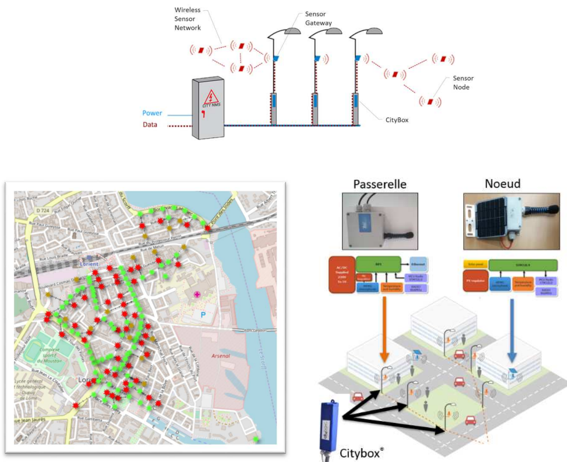
Figure 2:3 Illustration of the CENSE network. Above: communication between sensor nodes, sensor gateways, and power supply. Bottom left: sensor network deployed. Bottom right: sensors deployed as part of the project and infrastructure diagram.
