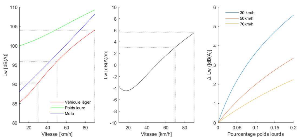
Figure 3:2 Emission laws relating to the IMAGINE model (Peeters & van Blokland, 2007). a) Sound power L_w (in dB(A)) as a function of speed; b) Difference in sound power per unit distance \Delta L_w (in dB(A)/m); c) Impact of the percentage of heavy vehicles on the sound power of the flow (in dB(A)).
