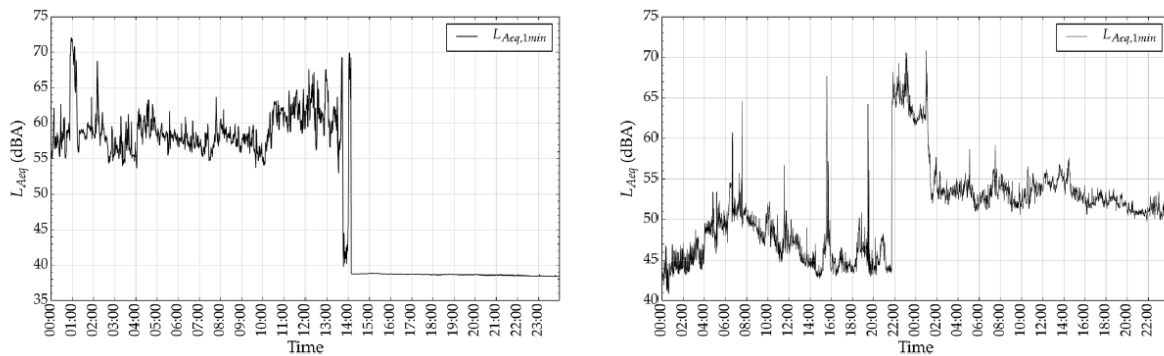
Figure 2:14 Example of microphone failure detection as performed in Dauwe et al. (2014). Left: microphone breakdown. Right: incipient failure (windshield detachment resulting in a background noise increase. Source: Dauwe et al. , 2014.
