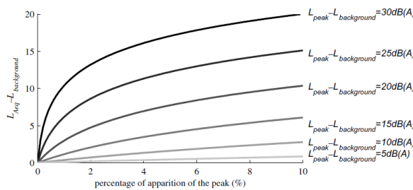
Figure 1:9 Influence of the duration and intensity of an emergence on the value of L_{Aeq} . Source: Can et al. (2008) .
