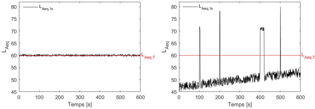
Figure 1:8 Two different L_{Aeq,1s} time series for the same L_{Aeq,T}
