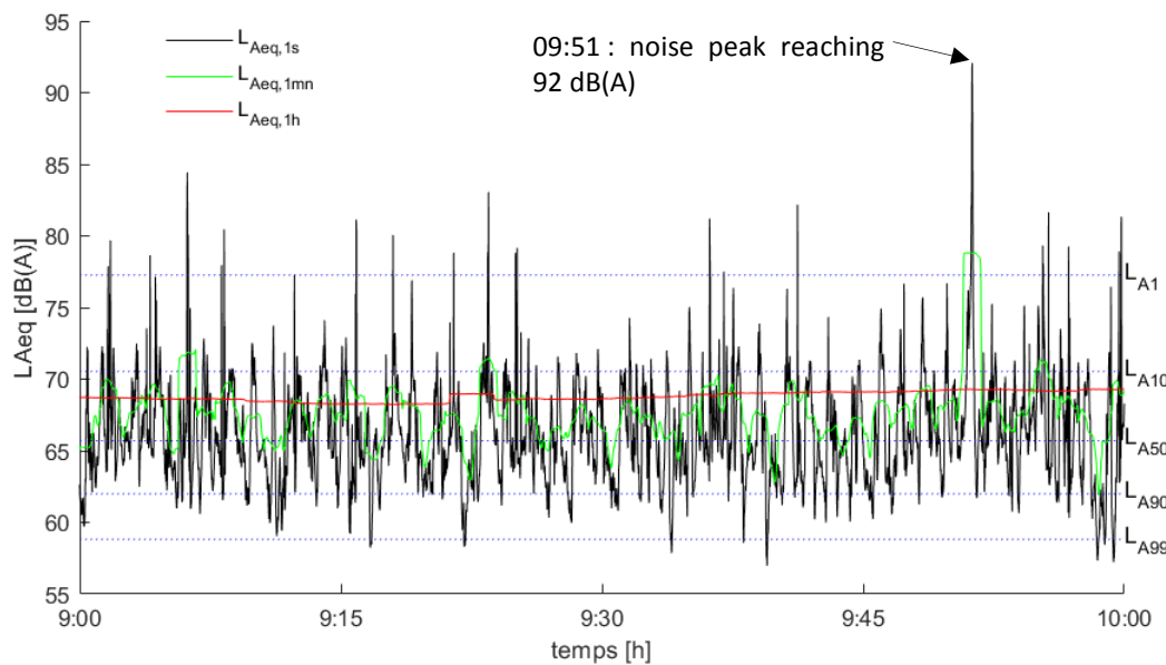
Figure 1:5 Evolution of the L_{Aeq,1s} at a Paris XIII measurement point, over a period of 1 hour (69 boulevard Auguste Blanqui, day of March 2, 2015), period [9:00-10:00]). Source of measurements: Lavandier et al. (2017) .
