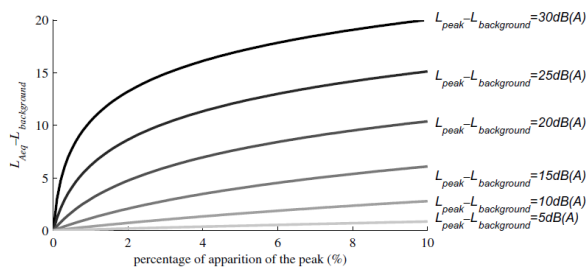
Figure 1:9 Influence of the duration and intensity of an emergence on the value of L_{Aeq} . Source: Can et al. (2008) .
