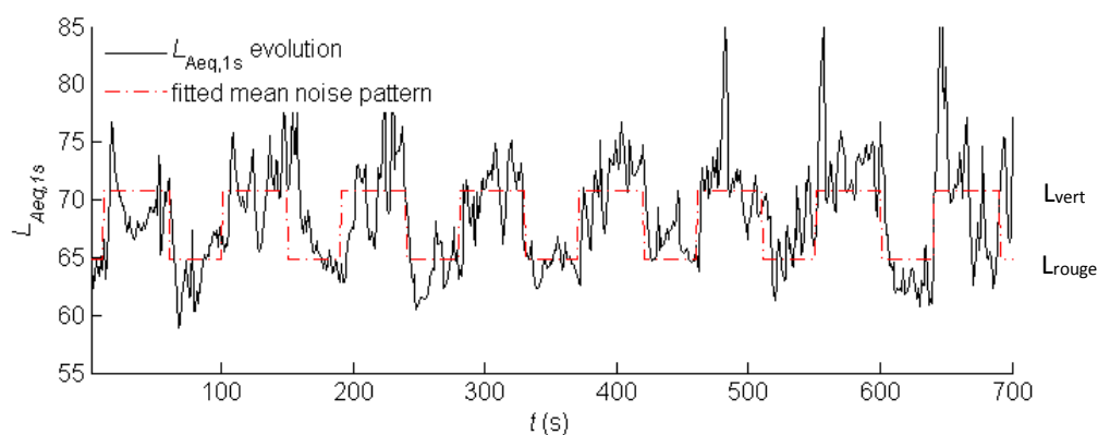
Figure 1:13 Time series of L_{\text{Aeq},1s} measured downstream of a traffic light and near a bus stop. Source: Can et al., 2010 .
