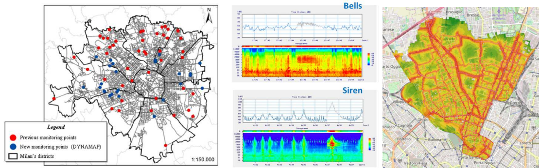
Figure 2:5 Illustration of the DYNAMAP network. Left: Measuring points. In the center: module for detecting abnormal events. On the right: example of a noise map produced. (Source: Zambon et al. , 2017).
