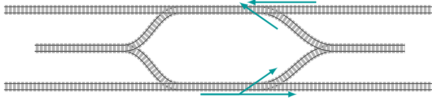
Figure 3.2: A junction (top) and a fork (bottom)
