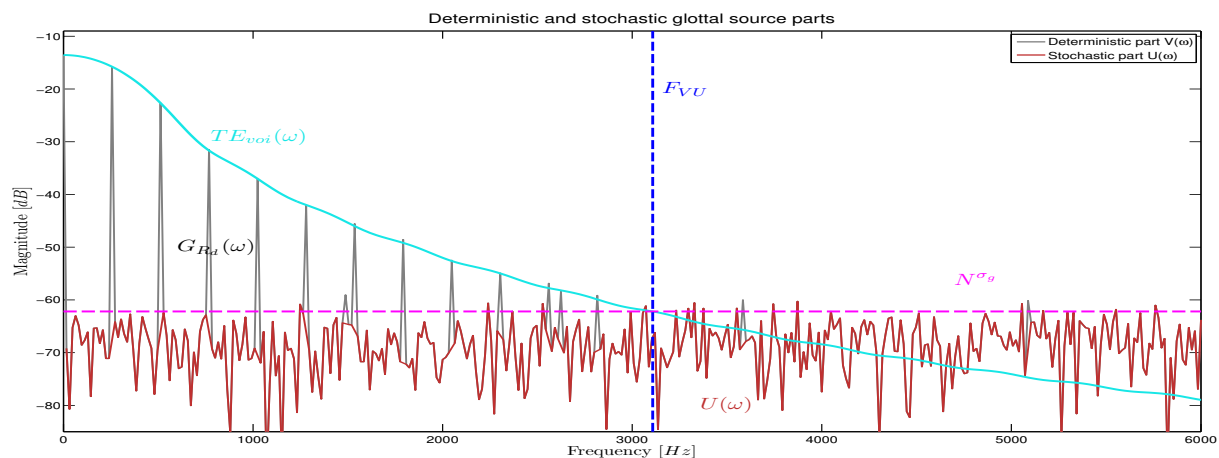
Figure 2.2: Synthetic example of the glottal excitation source
