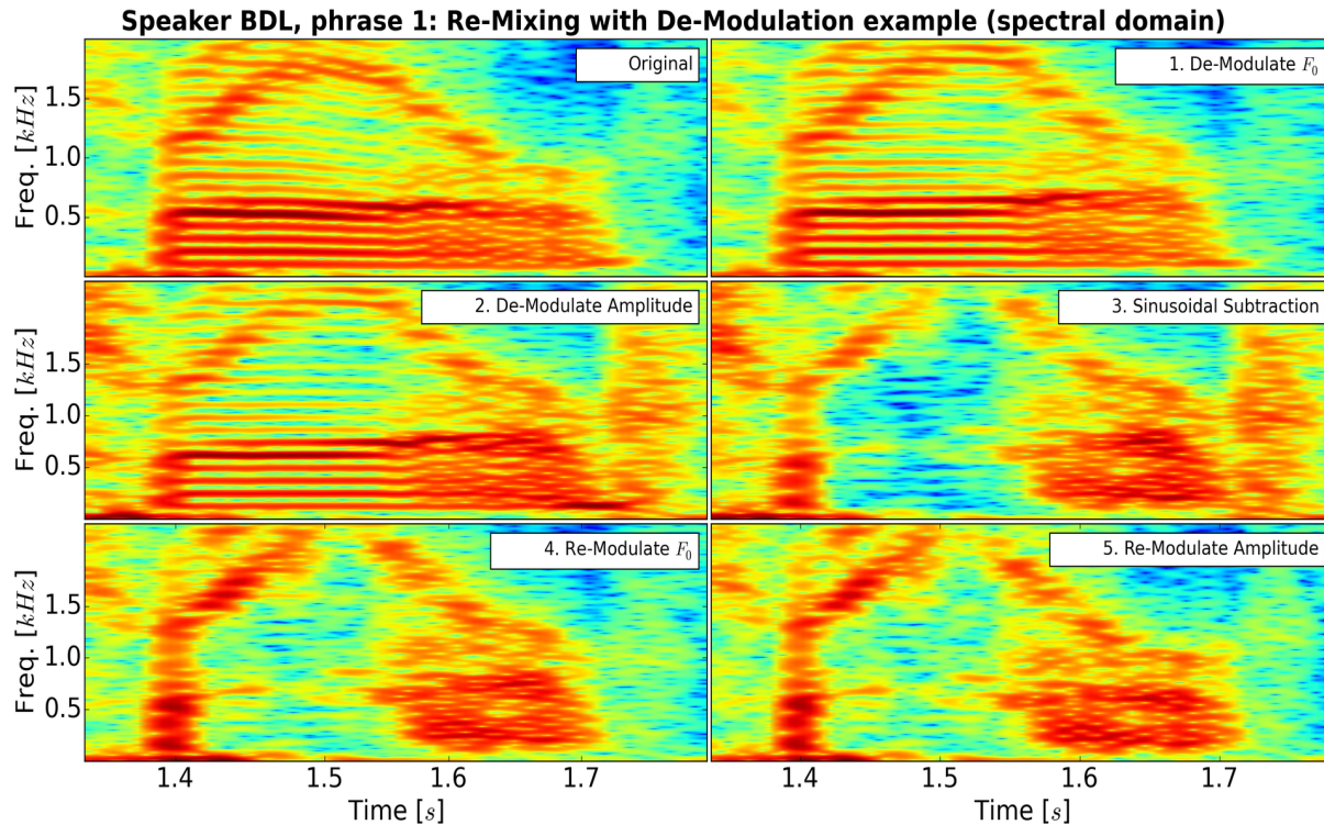
Figure 6.18: Spectral example of "Re-Mixing with De-Modulation" to estimate U_{ReDe}^{AMFM}(\omega)
