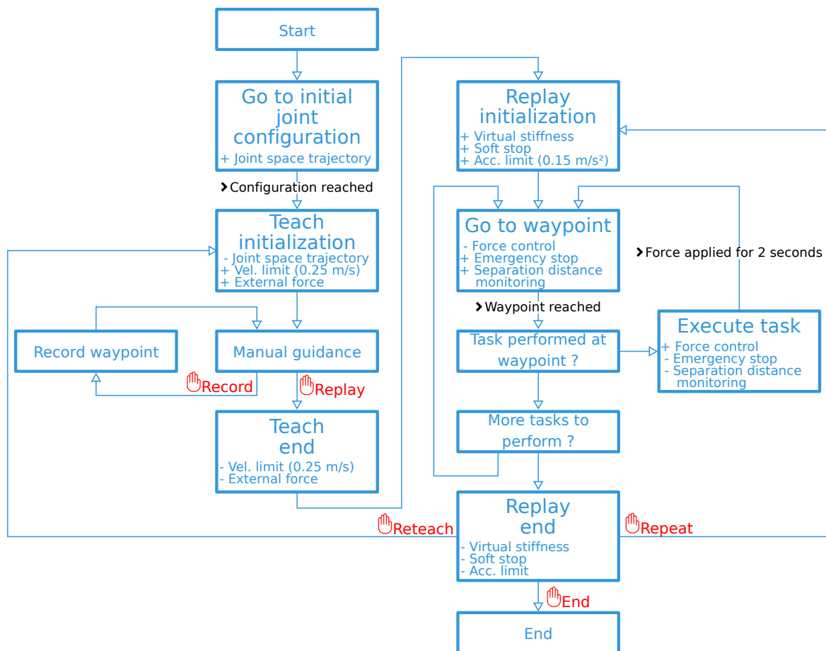
Figure 3.12 The FSM used for the experiment. A plus sign indicates an addition to the controller (a new constraint or new input) while a minus indicates a removal.
