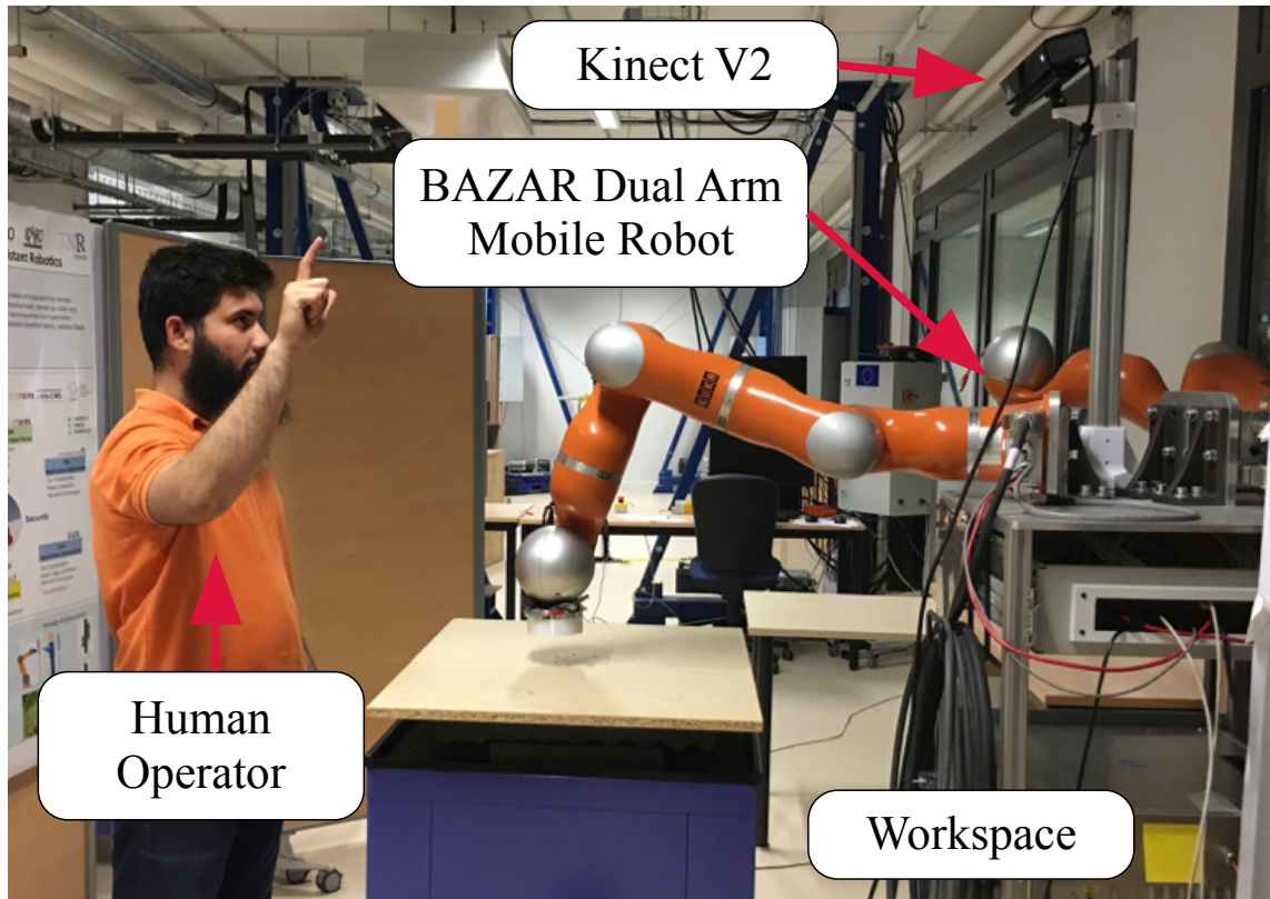
Figure 3.11 Safe Physical Human Robot Interaction Setup
