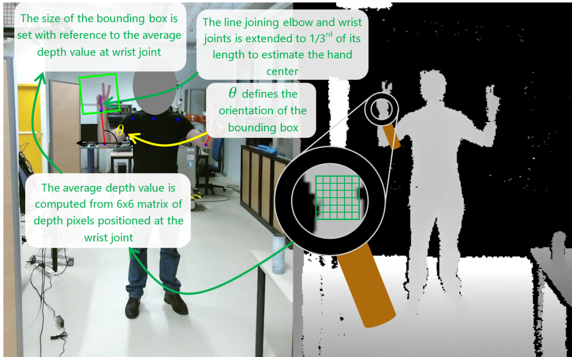
Figure 3.2 Localization of hand through openpose is illustrated. The bounding box is titled with an angle that the forearm makes with horizontal, while the size of bounding box is determined by the mean depth value of the wrist joint. The mean depth value is computed by averaging the depth pixel values of a 6 \times 6 matrix centered at the wrist joint.
