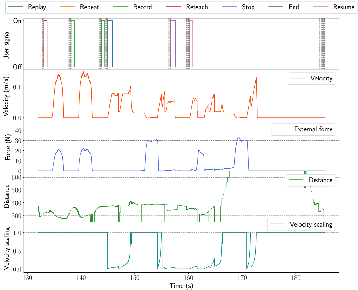
Figure 3.14 Experimental results. From top to bottom: hand gesture detection (dashed lines correspond to detection instants and plain line to the activation signals), control point translational velocity, external force at the end-effector, distance between the camera and the closest human body part and velocity scaling factor computed by OpenPHRI to slow down the motion.
