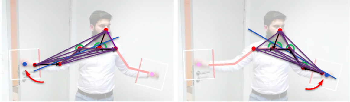
Figure 4.6 Illustration of augmented pose vector features for hands bounding boxes size estimation.
