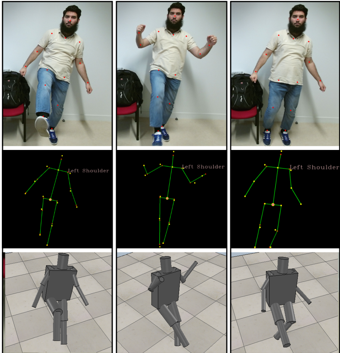
Figure 5.4 3D pose estimations with full-body articulations. It can be seen that proposed strategy fails to solve depth ambiguity for (lower) limbs movements in saggital plane. Also the optimization falls into local minima in some cases as shown.
