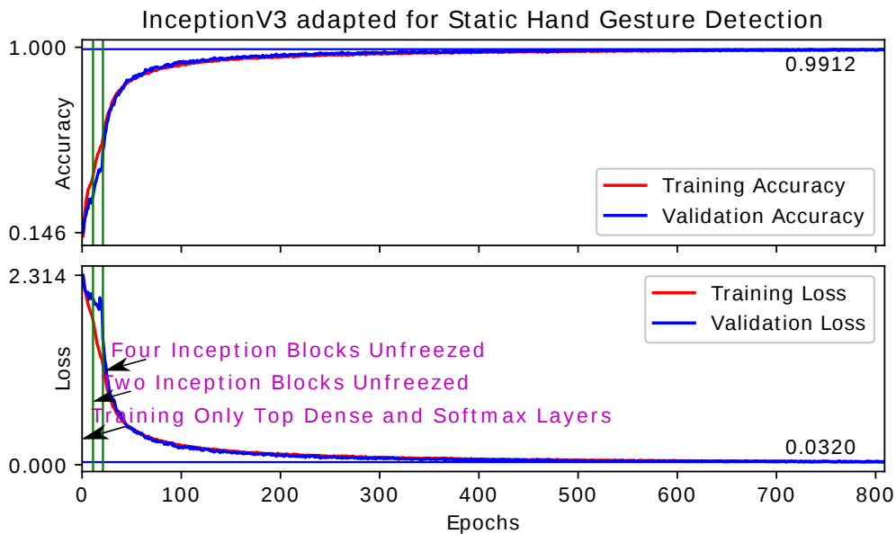
Figure 3.9 Plot of validation accuracy (top) and validation loss (bottom)
