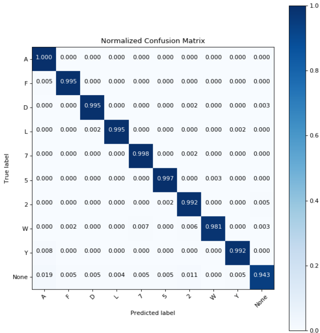
Figure 3.10 Normalized Confusion Matrix Quantified on Test-Set
