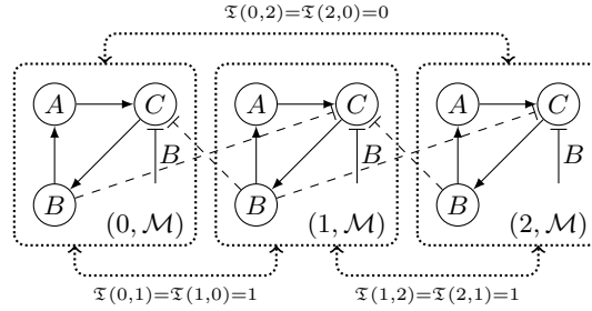
Fig. 31. A CLRMS (\mathfrak{J}, \mathfrak{M}, \mathfrak{T}) encompassing three copies of the LRM \mathcal{M} from figure 30, where: \mathfrak{J} \stackrel{\text{df}}{=} \{0, 1, 2\} , \mathfrak{M} \stackrel{\text{df}}{=} \{(0, \mathcal{M}), (1, \mathcal{M}), (2, \mathcal{M})\} , and \mathfrak{T} \stackrel{\text{df}}{=} \{(0, 1) \mapsto 1; (1, 2) \mapsto 1; (2, 0) \mapsto 0\} completed symmetrically. Functions \varphi_{B,C} in modules 0 and 1 depend on the level of B in module 1 (the sole connected module containing B ) whereas \varphi_{B,C} in module 1 depends on the levels of B in both modules 0 and 2.
