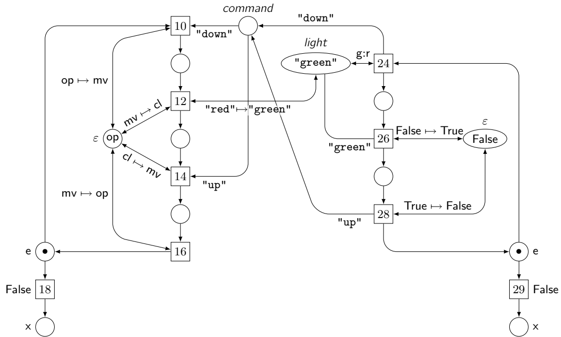
Fig. 13. The semantics of \text{gates}() \mid \text{track}() , where \text{op} \stackrel{\text{df}}{=} \text{"open"} , \text{cl} \stackrel{\text{df}}{=} \text{"closed"} , \text{mv} \stackrel{\text{df}}{=} \text{"move"} and \text{g:r} \stackrel{\text{df}}{=} (\text{"green"} \mapsto \text{"red"}) . The unlabelled places are internal ones. The anonymous place marked by \text{op} implements buffer state of net \text{gates} . The anonymous place marked by \text{False} implements buffer crossing of net \text{track} . Transition names correspond to the line numbers of the atomic actions they implement.
