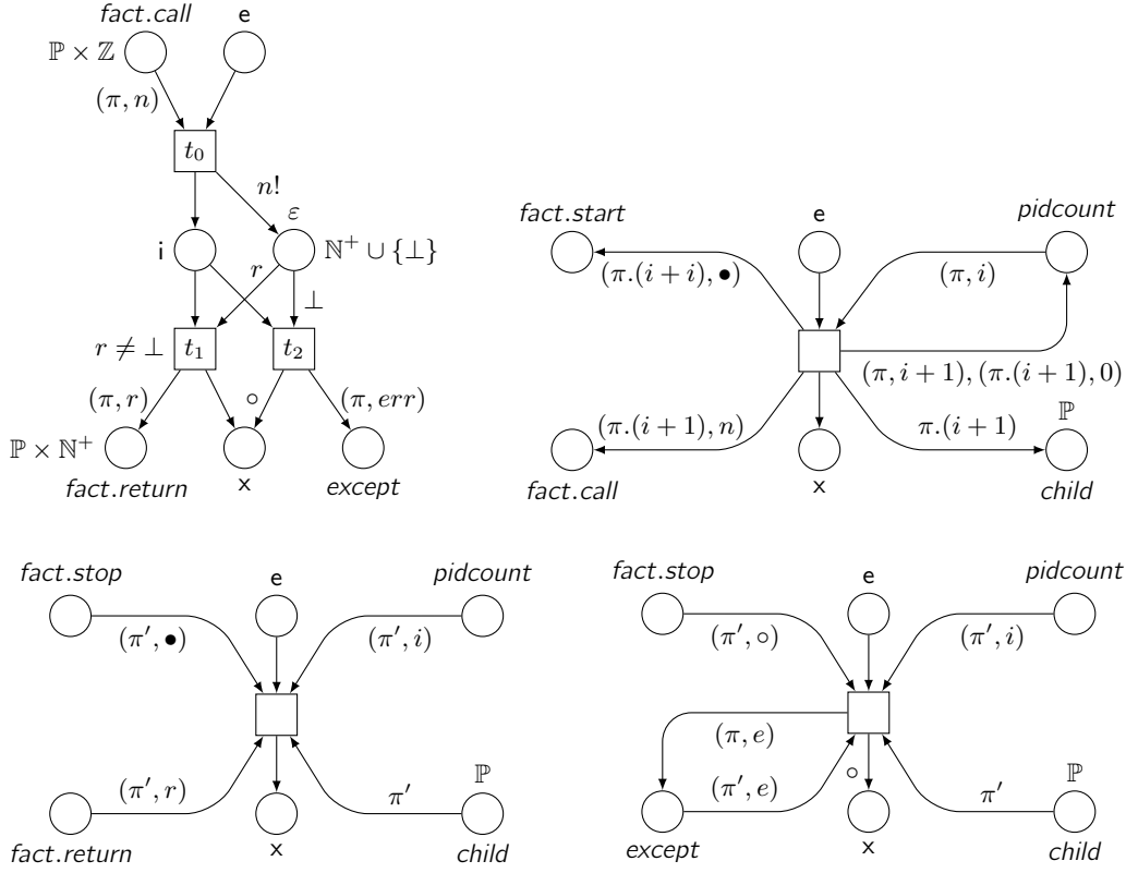
Fig. 19. Top left: the implementation of function fact , where err is a suitable error value. Top right: a sub-net N_c that calls fact(n) where n \in \mathbb{Z} . Bottom left: a sub-net N_r that waits for fact to return. Bottom right: a sub-net N_e that waits and propagate an exception from fact . As usual, labels \{\bullet\} on arcs have been omitted.
