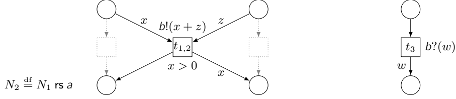
Fig. 8. The result of the restriction with respect to a of the net N_1 from figure 6; transitions t_1 and t_2 (indicated in dotted gray lines) have been removed.
