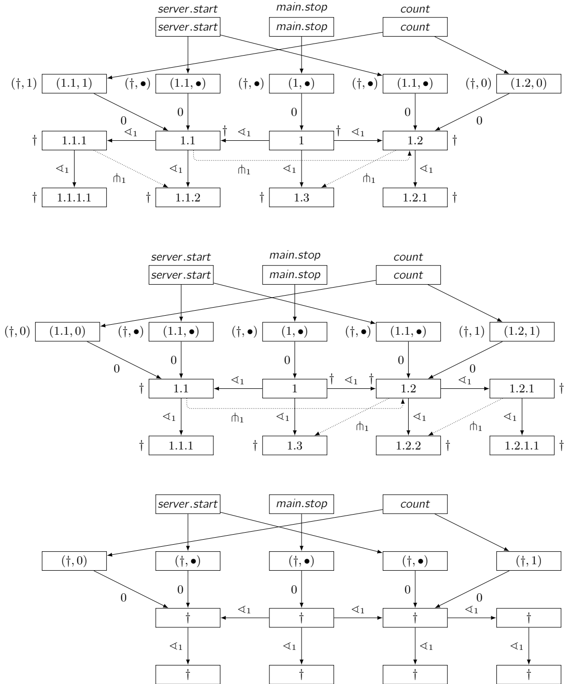
Fig. 23. Top: the graph representation of state 2 from figure 22. Middle: the graph representation of state 3. Bottom: the graph representation of both states when \hat{m}_1 \notin \Omega_{pid} , where nodes identities have been replaced by nodes labels.
