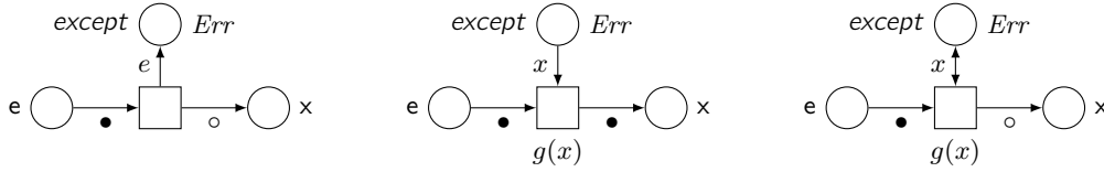
Fig. 16. Left: net R_e that raises an exception with value e \in \text{Err} . Middle: net C_g that catches an exception value according to a Boolean function g . Right: net P_g that catches and propagates an exception value according to a Boolean function g .
