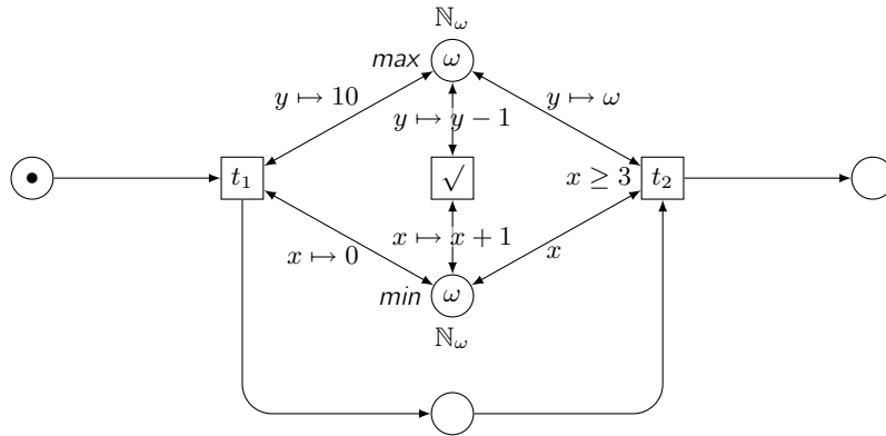
Fig. 25. A simple causally timed system with two counters \min and \max and a tick transition \sqrt{\phantom{x}} . Transition t_2 must fire when at least 3 and at most 10 ticks have occurred since t_1 has fired.
