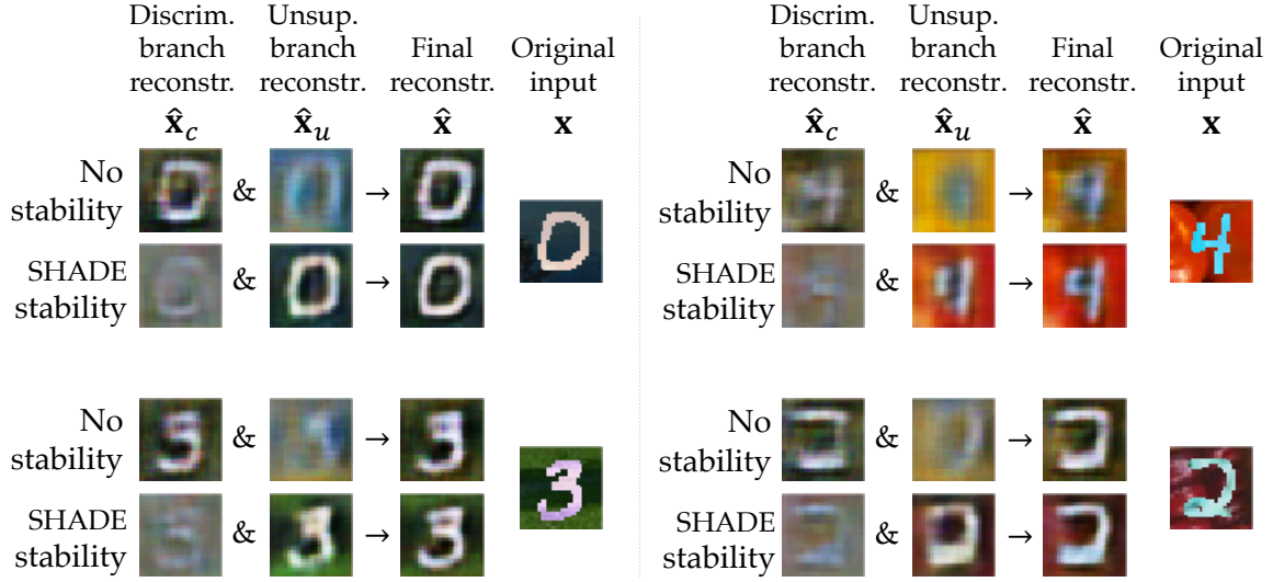
Figure 3.8. – Reconstructions of samples from MNIST-M by HybridNet with and without SHADE . We show the final reconstruction \hat{x} = D(\mathbf{h}) = D(\mathbf{h}_c + \mathbf{h}_u) and the “partial” reconstructions \hat{x}_c = D(\mathbf{h}_c) and \hat{x}_u = D(\mathbf{h}_u) produced when feeding the decoder with the features from a single branch.
