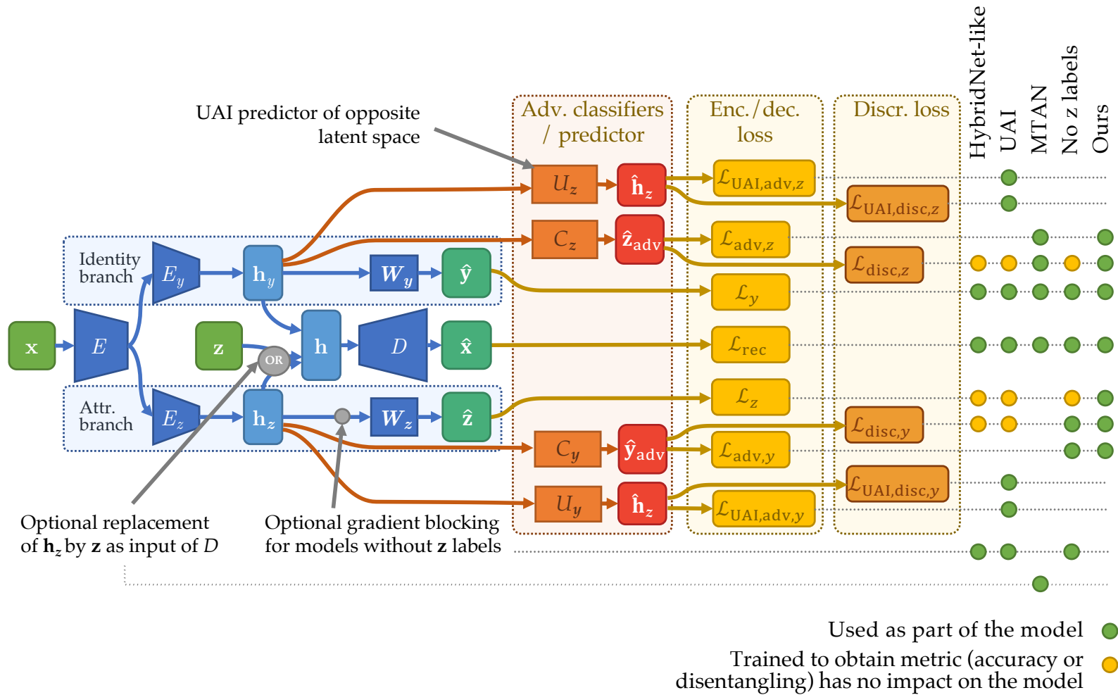
Figure C.1. – Complete architecture with all possible options and variants. We also show which loss terms are activated to reproduce the different models that we report.
