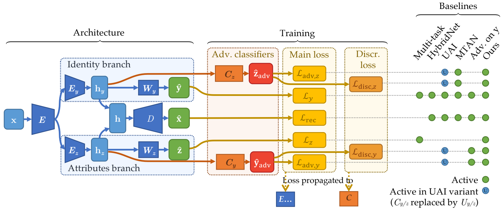
Figure 4.4. – Architecture and learning of the DualDis framework. We use a two-branch encoder-decoder architecture with classifiers (left). For the training, in addition to classical reconstruction and classification losses, we use adversarial classifiers and loss terms to force the two latent spaces to encode complementary “orthogonal” information (middle). We also indicate (right) how subsets of components of DualDis can be used to reproduce existing baselines described in Section 4.4, in particular Multi-task models (Kokkinos 2017), HybridNet, UAI (Jaiswal et al. 2018), MTAN (Yang Liu et al. 2018), models with an adversarial loss on y only (Hadad et al. 2018; Yu Liu et al. 2018; Klys et al. 2018).
