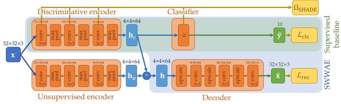
Figure 3.7. – Detailed architecture of an HybridNet trained with SHADE. We indicate the supervised baseline (delimited in green), SWWAE (delimited in blue) and HybridNet (whole figure) used for MNIST-M.
