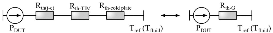
Fig. 3-4. Global thermal resistance.
