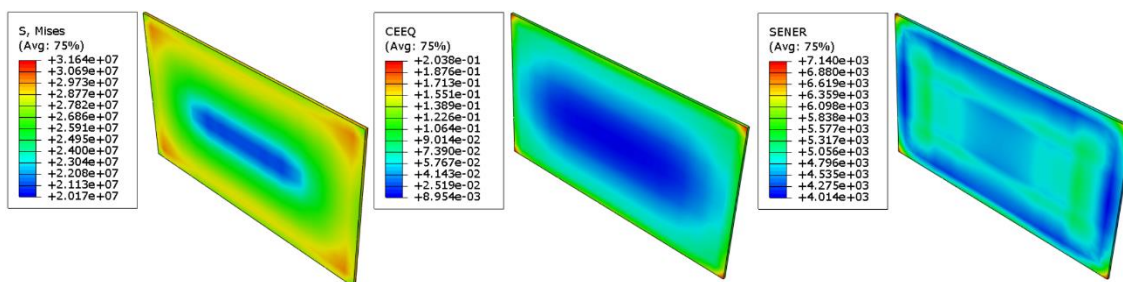
Fig. B-2. Accumulated strain, strain energy and stress distributions in the solder joint.
