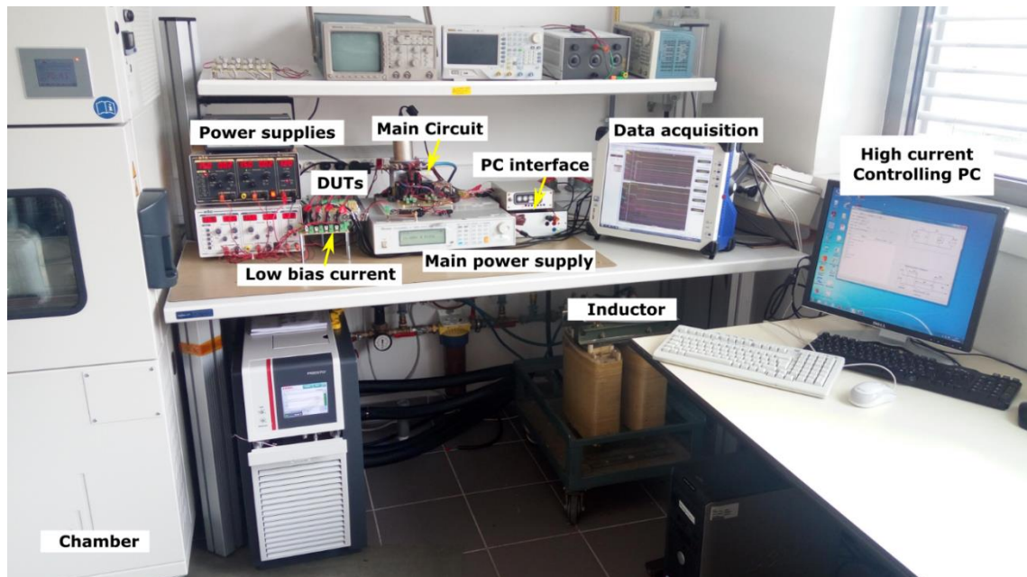
Fig. 3-5. Implemented test bench for power cycling and thermal cycling accelerated aging tests.
