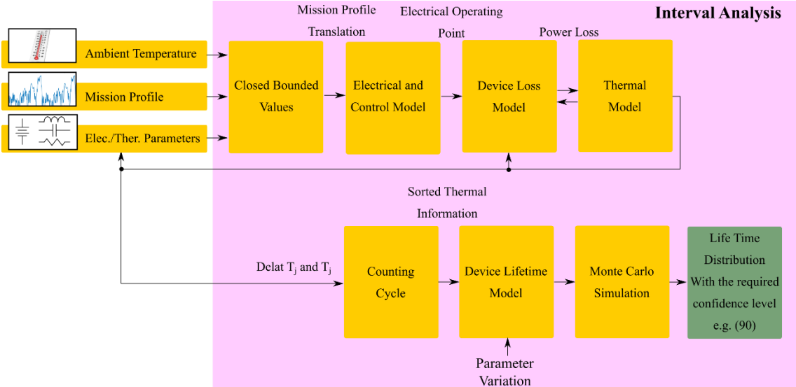
Fig. 5-11. New algorithm of interval reliability assessment for converters.
