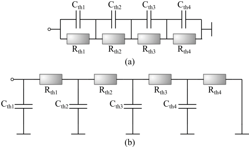
Fig. 2. 19. Thermal model. (a) Foster model, (b) Cauer model.
