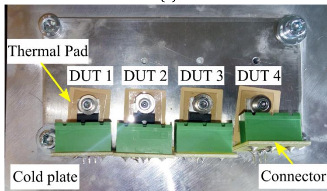
Fig. 3-3. Devices under test. a) Schematic circuit of IGBTs and diodes under test, b) mounted DUTs on cold plate
