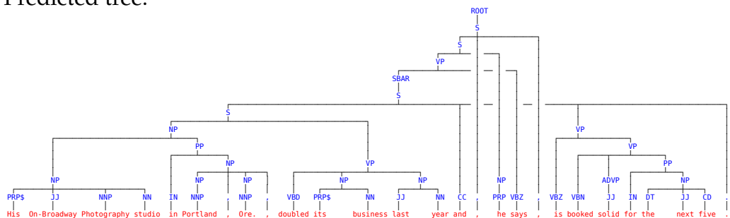
Figure 8.8: Partially recognized circumpositioned quotations.
