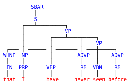
Figure 8.4: Partial recognition cases for wh-extractions: extraction site errors.
