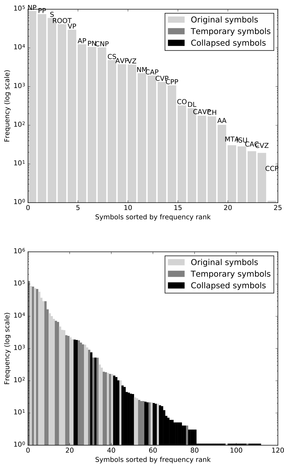
Figure 3.5: Symbol distribution in the Tiger treebank before (upper part) and after (lower part) preprocessing.
