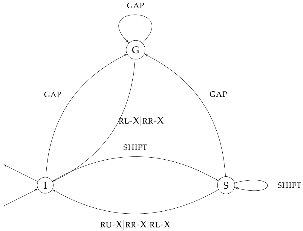
(a) SHIFT-REDUCE-COMPOUND-GAP
