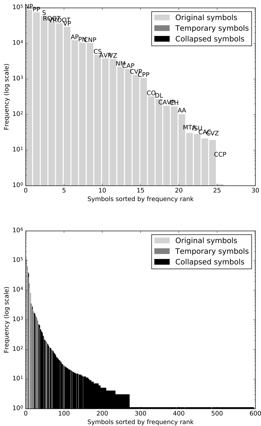
Figure 3.6: Symbol distribution in the SPMRL projectivized version of the Tiger treebank, before (upper part) and after (lower part) preprocessing.
