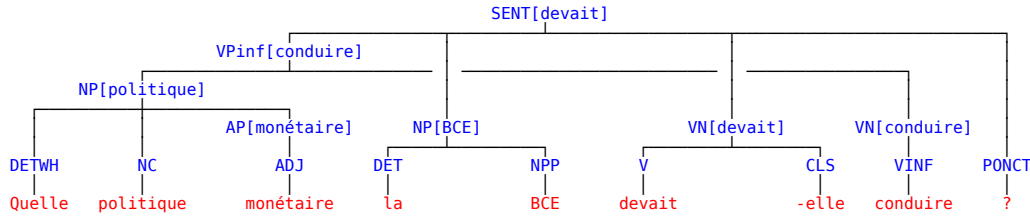
Figure 1.3: Lexicalized Constituency Tree.
