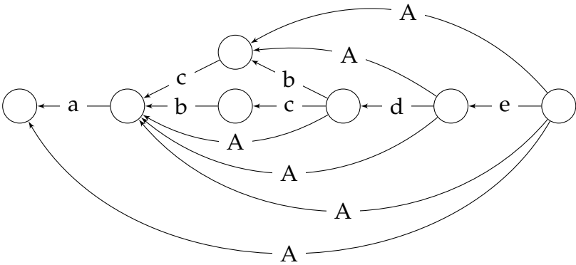
(a) GSS encoded in the search space with backpointers.
