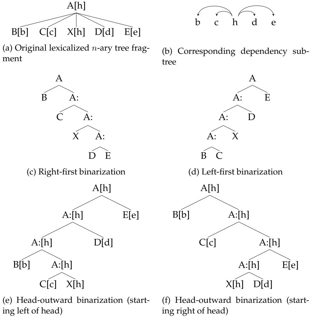
Figure 3.4: Four binarization strategies.
