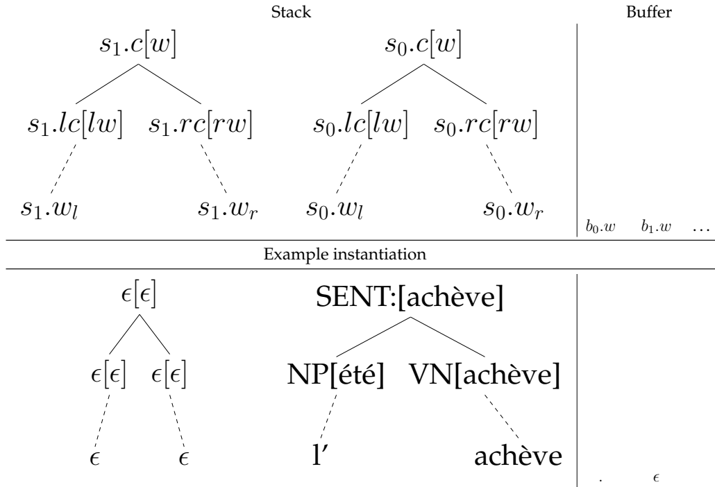
Figure 4.2: Illustration of the locality of an abstract configuration and a concrete configuration when deriving the tree in Figure 3.1 (lower left-hand part).
