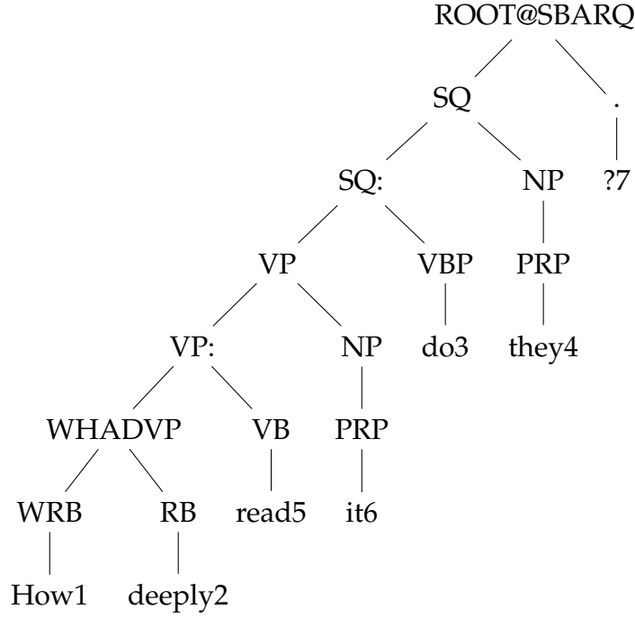
Figure 7.6: Projective tree obtained from the tree in Figure 7.2 by reordering terminals.
