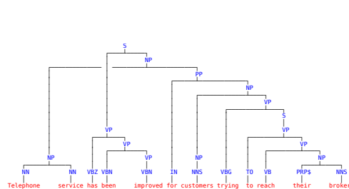
Figure 8.7: Non-detected extrapositions.
