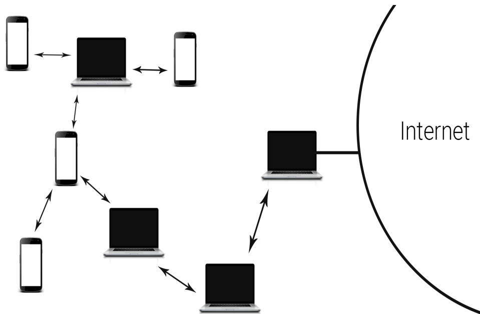
Fig. 2.2 Example of Mobile Ad Hoc Network (MANET) [57]
