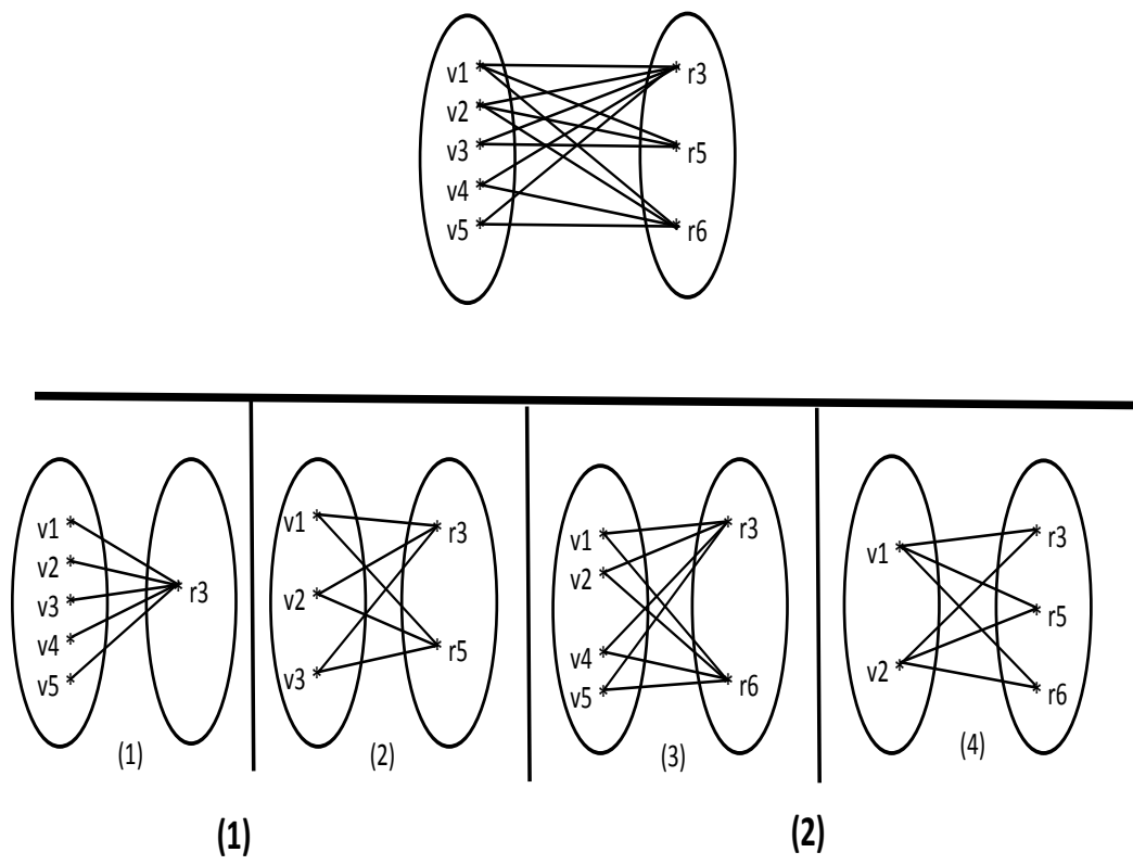
Fig. 3.3 Pseudo-concept
