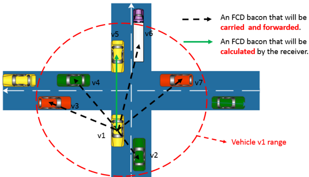
Fig. 4.4 Urban scenario case
