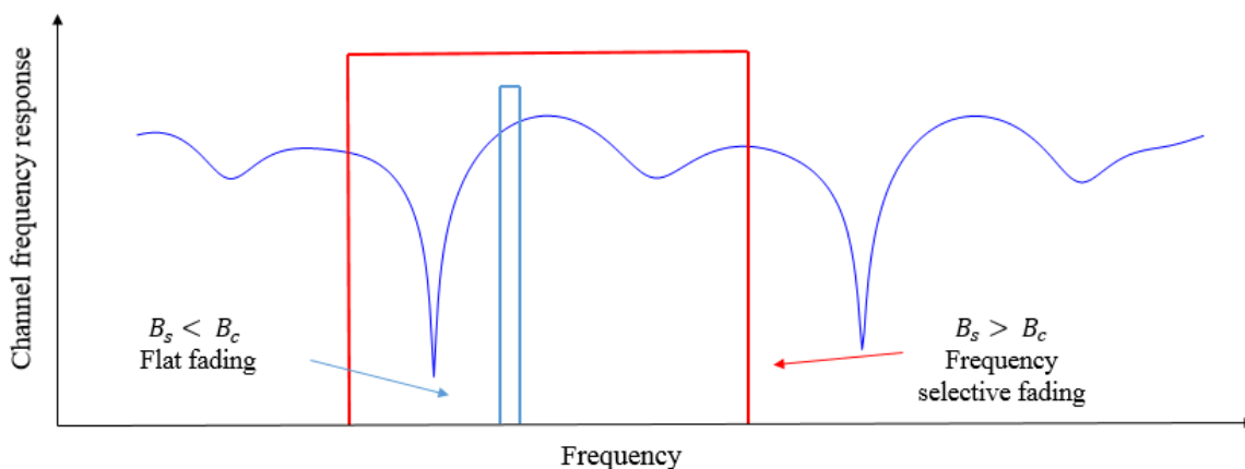
Figure 1.6: Flat fading vs Frequency selective fading
