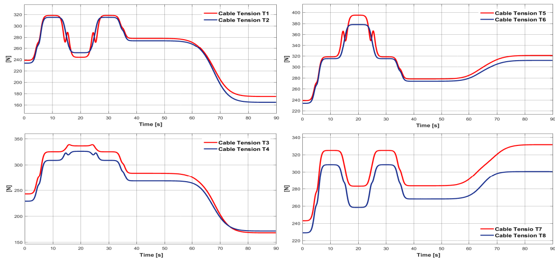
FIGURE 4.12: Cables tension
