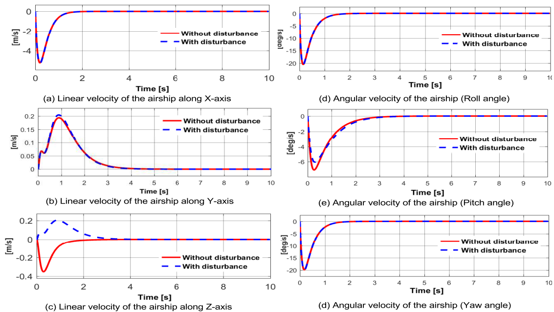
FIGURE 6.5: Linear and angular velocity of the airship with and without disturbance
