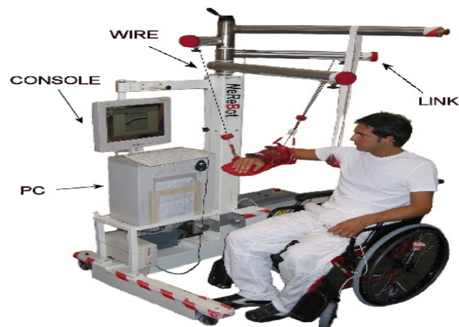
FIGURE 1.5: NeReBot for rehabilitation
