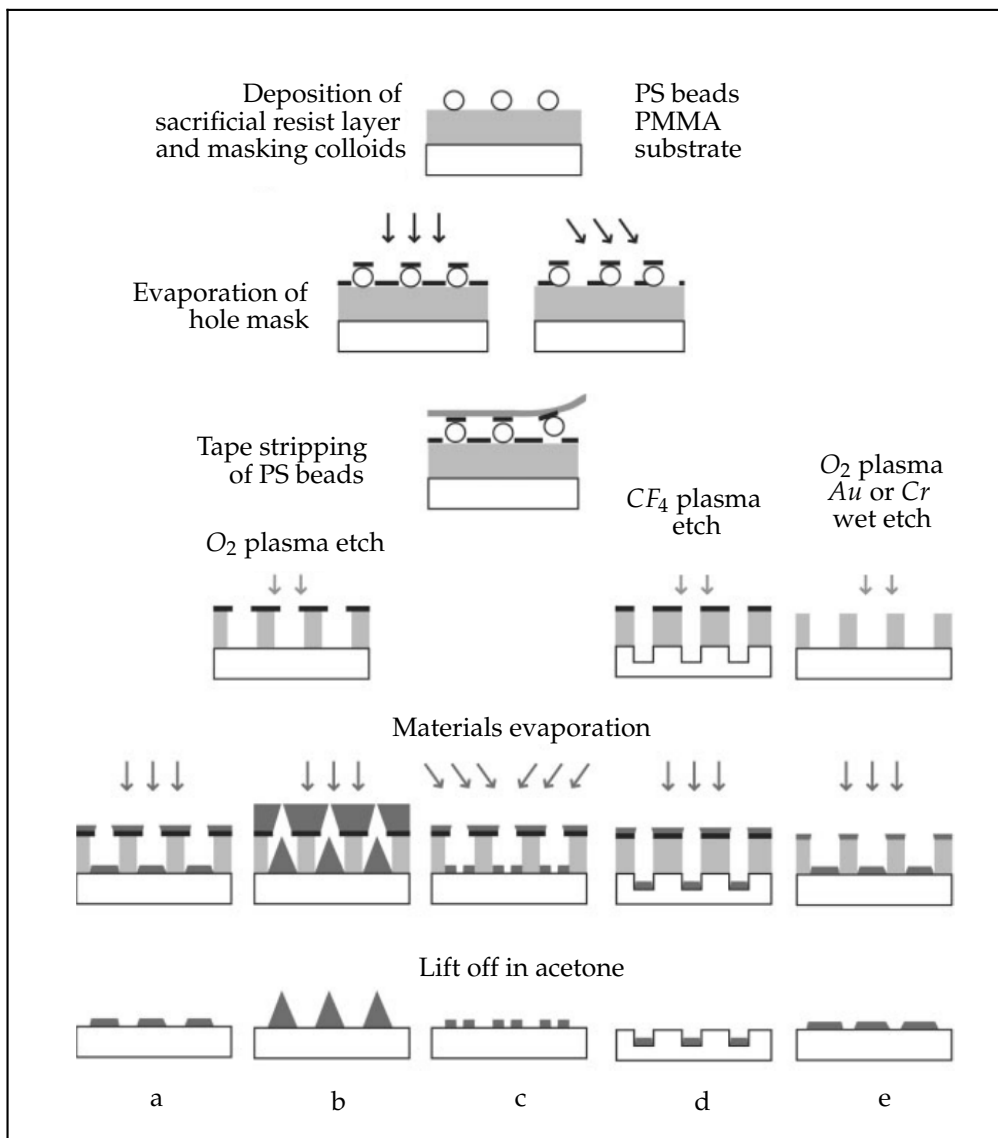
FIGURE 3.2: Diagram illustrating the basic steps and resulting structures produced with hole-mask colloidal lithographie. The resulting structures are a. arrays of nanodiscs and oriented elliptical nanostructures, b. nanocone arrays, c. binary arrays of nanodisc pairs, d. embedded nanodiscs, and e. discs with fine tunable diameters. The diagram was taken from ref. [iii7].
