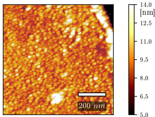
FIGURE 4.4: AFM image of Au evaporated on glass using OAD. The particles show an average height of 10\text{nm} . However, no information can be extracted from this image regarding the average width of the particles. Indeed, due to tip convolution, the particles appear larger than they really are. Moreover, the apparent shape of the particle being strongly dependent on the tip morphology, it is not possible to determine an overall orientation of the particles.
