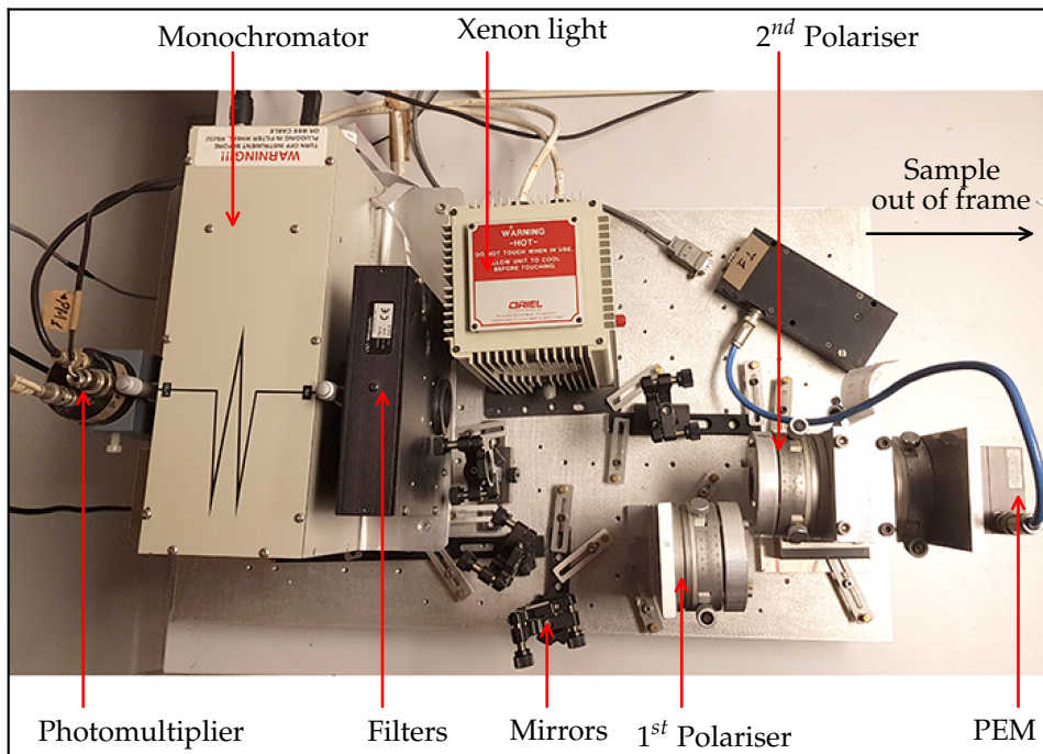
FIGURE 2.3: Photography of the RAS system with the different components indicated. The sample is placed on the far right of the system out of the frame.
