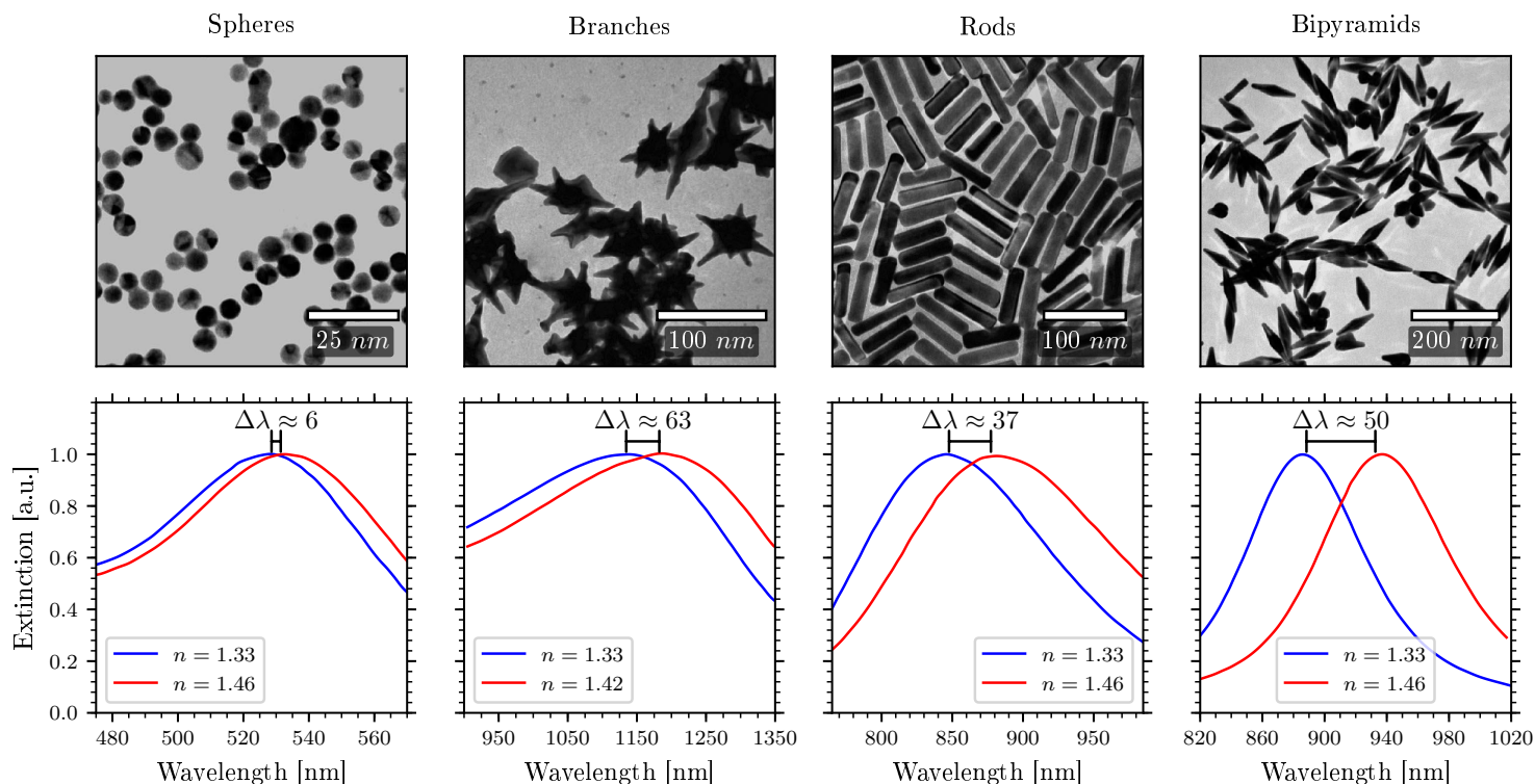
FIGURE 1.35: SEM images and there respective extinction spectra taken from ref. [i54]. The spectra are measured with non polarised light but at two different refractive index. These were obtained by adding different amount of glycerol in water. For the rods and bipyramids only the resonance at higher wavelength is shown.
