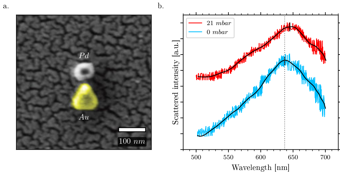
FIGURE 5.7: a. SEM image from ref [v31]. b. Scattering spectrum of system a. under vacuum and under 21mbar of H 2 from the same reference.
