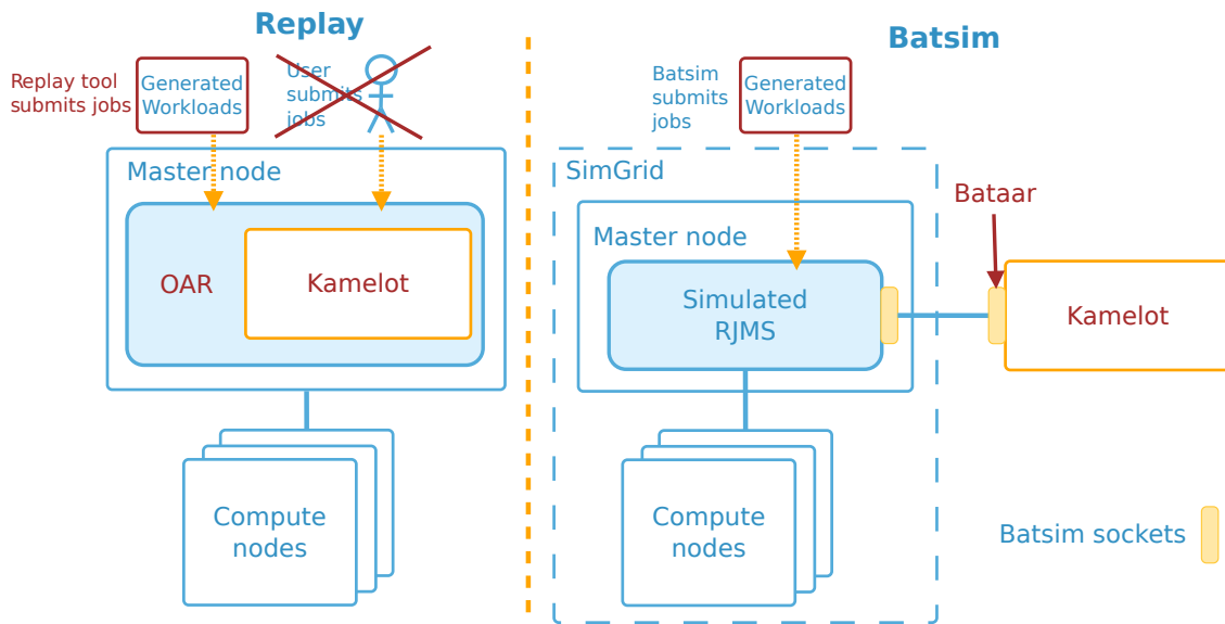
Figure 6.3.: Batsim validation process using a real world Resource and Job Management System scheduler.
