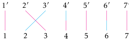
FIGURE 3. If p = q , the same link can be coloured with two different colors. We draw in cyan the links coloured with + and in magenta the links coloured with -.
