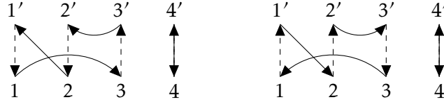
FIGURE 6. Two orientations of the same Brauer diagram
