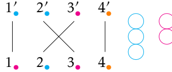
FIGURE 7. A diagram with loops.
