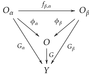
FIGURE 26. Universal property of the inductive limit.
