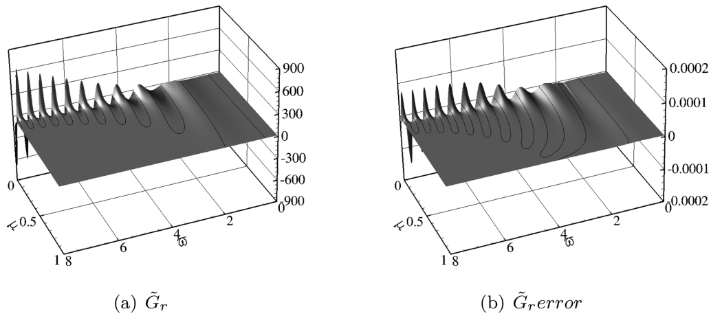
Fig. 3. Results for the evaluation of \tilde{G}_r and error with the direct integration method. The ODE is solved using the RK4 method with \Delta\omega = 0.001 \omega \in (0, 8] , and \mu \in [0, 1] .
