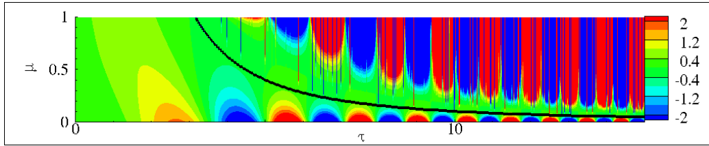
(c) \Delta\mu = 0.0001
