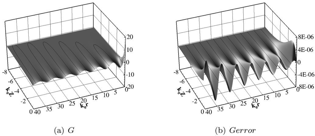
Fig. 4. Results for the evaluation of G and error with the direct integration method. The ODE is solved using the RK4 method with \Delta\omega = 0.001 .
