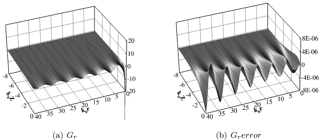
Fig. 5. Results for the evaluation of G_r and error with the direct integration method. The ODE is solved using the RK4 method with \Delta\omega = 0.001 .
