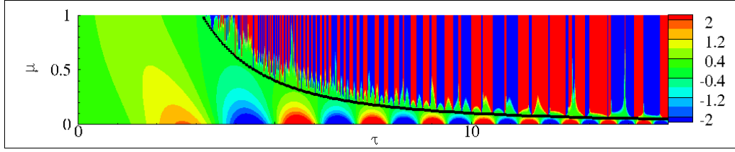
(a) \Delta\mu = 0.01
