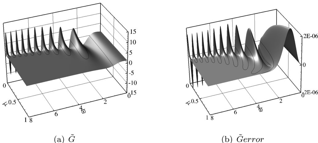
Fig. 2. Results for the evaluation of \tilde{G} with the ODE and error with the direct integration method. The ODE is solved using the RK4 method with \Delta\varpi = 0.001 \varpi \in (0, 8] , and \mu \in [0, 1) .
