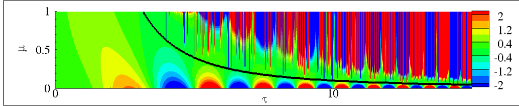
(b) \Delta\mu = 0.001
