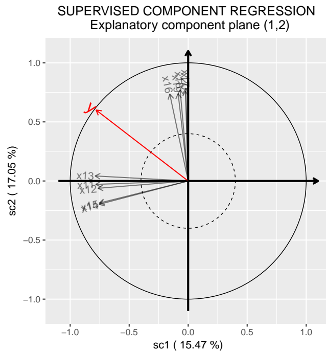
Figure 2.2 – Interpretative power of the SC regression. Using the same data, we present the component plane (1, 2) issued from the Supervised Component Regression. For an easier model interpretation, the explanatory variables having a cosine below 0.4 with the component plane are hidden.
